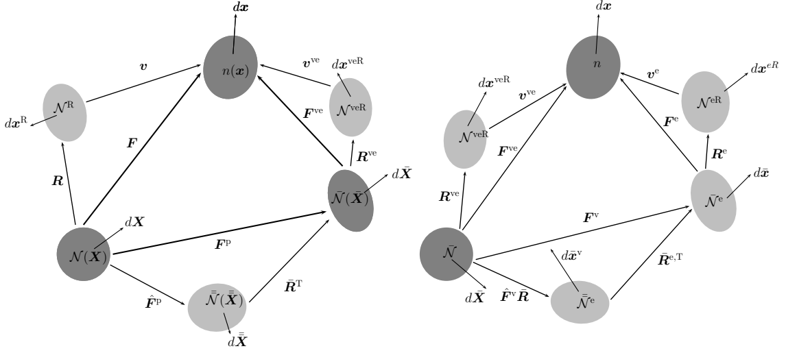
Figure 1: Deformation of a solid body in terms of the mappings between different placements (configurations): \mathcal{N} , \tilde{\mathcal{N}} , n , \mathcal{N}^R , and \mathcal{N}^{\text{veR}} for total viscoelastic-viscoplastic deformation (left) and \tilde{\mathcal{N}}^{\text{e}} , \tilde{\mathcal{N}}^{\text{v}} , and \mathcal{N}^{\text{eR}} for solely viscoelastic deformation split into an elastic (small deformations) and a viscous part (right). The symbols accentuated by the bar(s) refer to intermediate placements.
