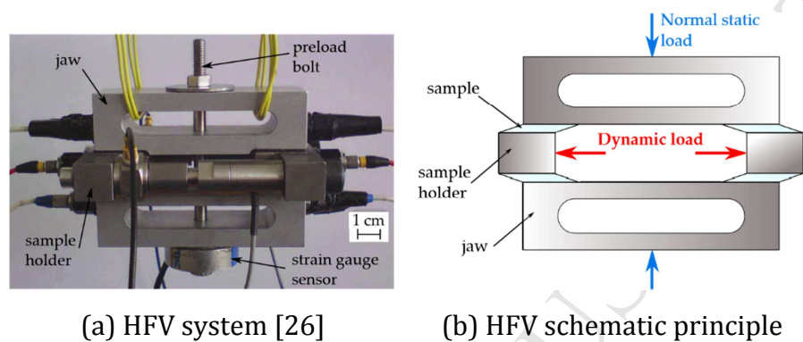
Figure 1: High-frequency viscoelasticity analyser.
