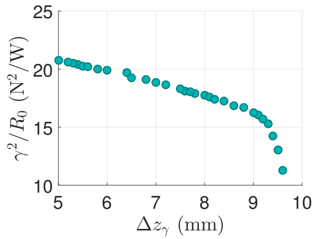
Figure C.3: Pareto-optimal solutions of the multiobjective optimization problem written in equation (C.3)
