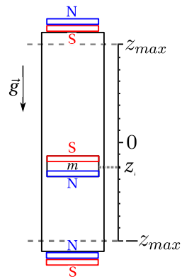
(b) Duffing with hardening nonlinearity
