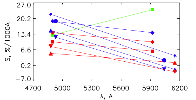
Fig. 3. Normalized reflectivity gradients of the selected NICs in the BV and VR spectral regions. Blue and red symbols indicate data points for the comets observed before and after perihelia, respectively; the target with a different spectral behavior is indicated in green.
