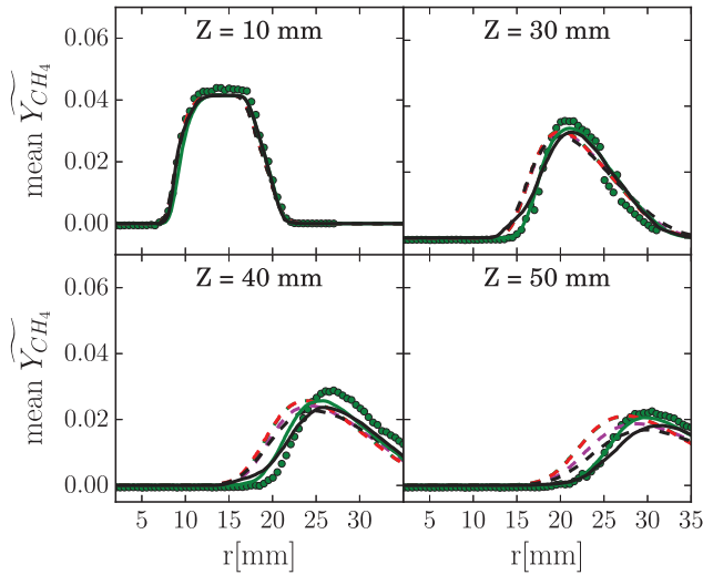
Fig. 23. 1-D radial profiles of the mean \text{CH}_4 mass fraction at different distances Z from the bluff-body wall surface. Legend: - - - 17M-FWF-N1, - - - 17M-FWF-N3, - - - 17M-FWF-NM, - - - 17M-FPF, — 135M-FWF-N1, — 135M-FPF, ● Experiments.
