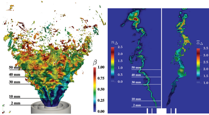
(a) Isosurface \overline{\dot{\omega}_c} = \max(\overline{\dot{\omega}_c})/2 colored by the fractal parameter \beta . (b) 2-D cut of n_\Delta (left) and \Xi_\Delta (right) scalar fields.
