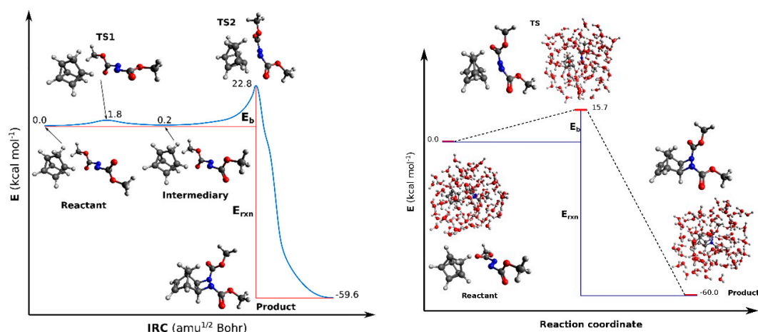
Figure 6. Reaction profile of quadricyclane with dimethyl azodicarboxylate in the gas and liquid phase (respectively, left and right panels).
