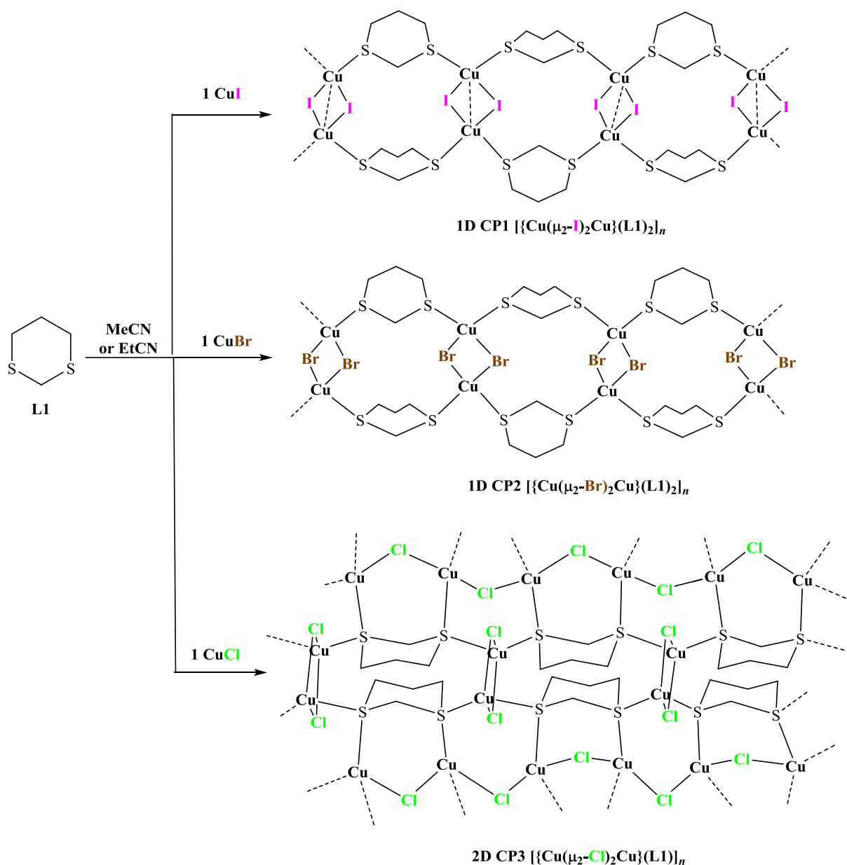
Scheme 1. Synthesis of the 1D CPs [\{\text{Cu}(\mu_2\text{-X})_2\text{Cu}\}(\mu_2\text{-L1})_2] CP1 ( X = \text{I} ) and CP2 ( X = \text{Br} ) and the 2D CP [\{\text{Cu}(\mu_2\text{-Cl})_2\text{Cu}\}(\mu_2\text{-L1})_2] CP3 .
