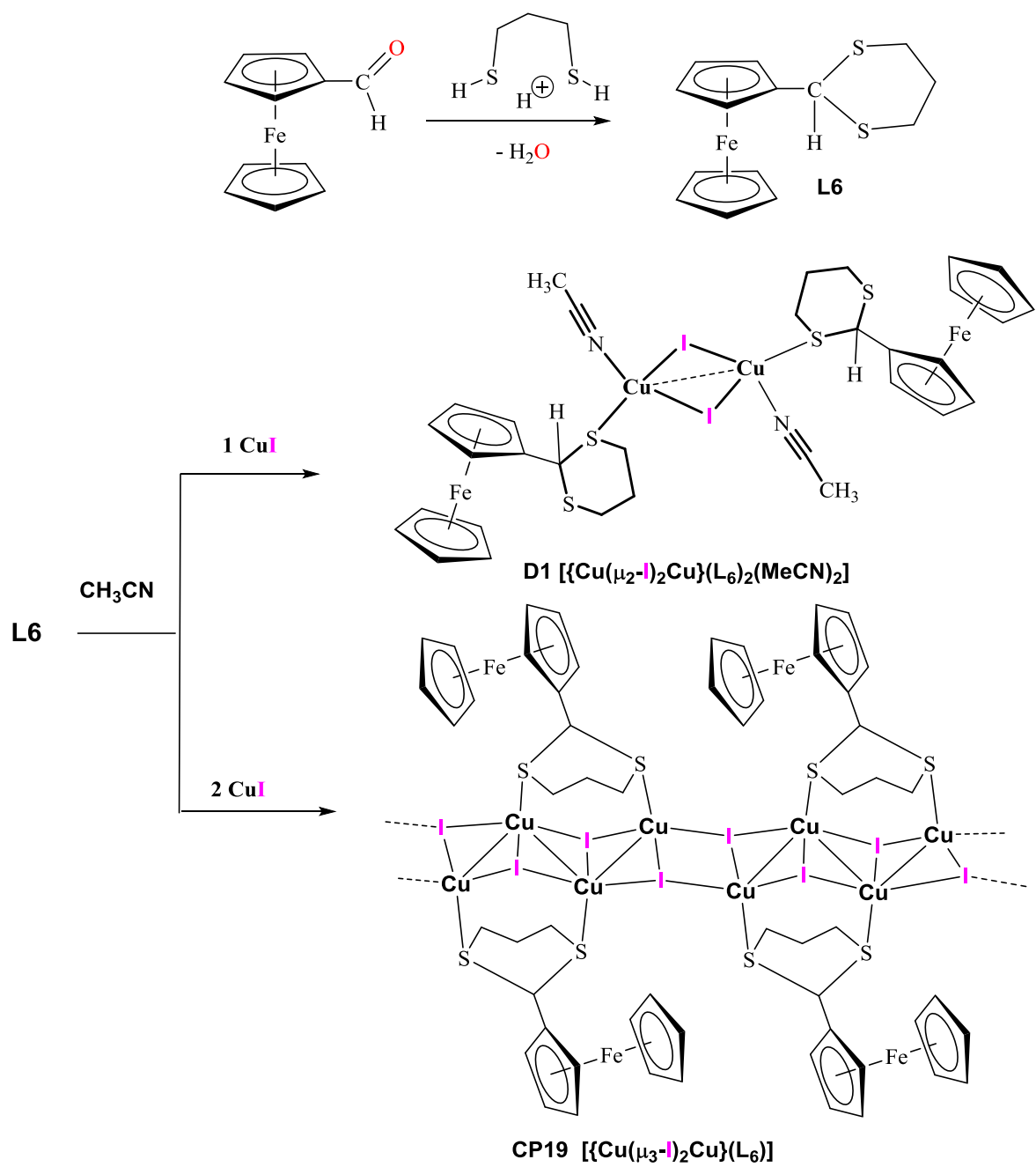
Scheme 7. Synthesis of L6 and its complexation on \text{CuI} yielding D1 and CP19 .
