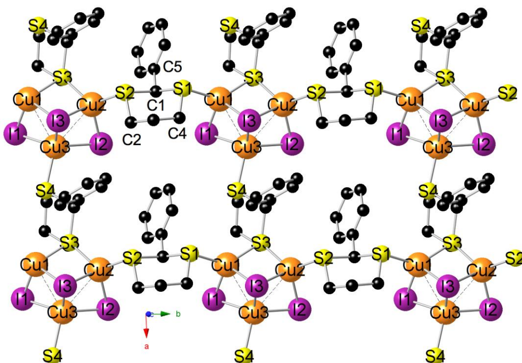
Figure 15. View on the a,b plane of the 2D network of [\{\text{Cu}_3(\mu_3\text{-I})(\mu_2\text{-I})_2(\mu_2\text{-L5})_2\}]_n CP17 . Selected bond lengths (Å) and angles ( ^\circ ): \text{Cu1-Cu3} 2.8302(4), \text{Cu2-Cu3} 2.8948(3), \text{Cu1}\cdots\text{Cu2} 3.297, \text{Cu1-I1} 2.5905(3), \text{Cu3-I1} 2.6591(3), \text{Cu1-I3} 2.7817(3), \text{Cu2-I3} 2.7803(3), \text{Cu3-I3} 2.6483(3), \text{Cu2-I2} 2.5842(3), \text{Cu3-I2} 2.6621(3), \text{Cu1-S1} 2.3050(3), \text{Cu1-S3} 2.3122(3), \text{Cu2-S2} 2.2876(5), \text{Cu2-S3} 2.2917(5), \text{Cu3-S4} 2.3393(5); \text{Cu1-I1-Cu3} 65.235(8), \text{Cu2-I2-Cu3} 66.961(8), \text{Cu1-I3-Cu2} 72.702(8), \text{Cu1-I3-Cu3} 62.771(8), \text{Cu2-I3-Cu3} 64.397(8), \text{Cu1-S3-Cu2} 91.461(16).
