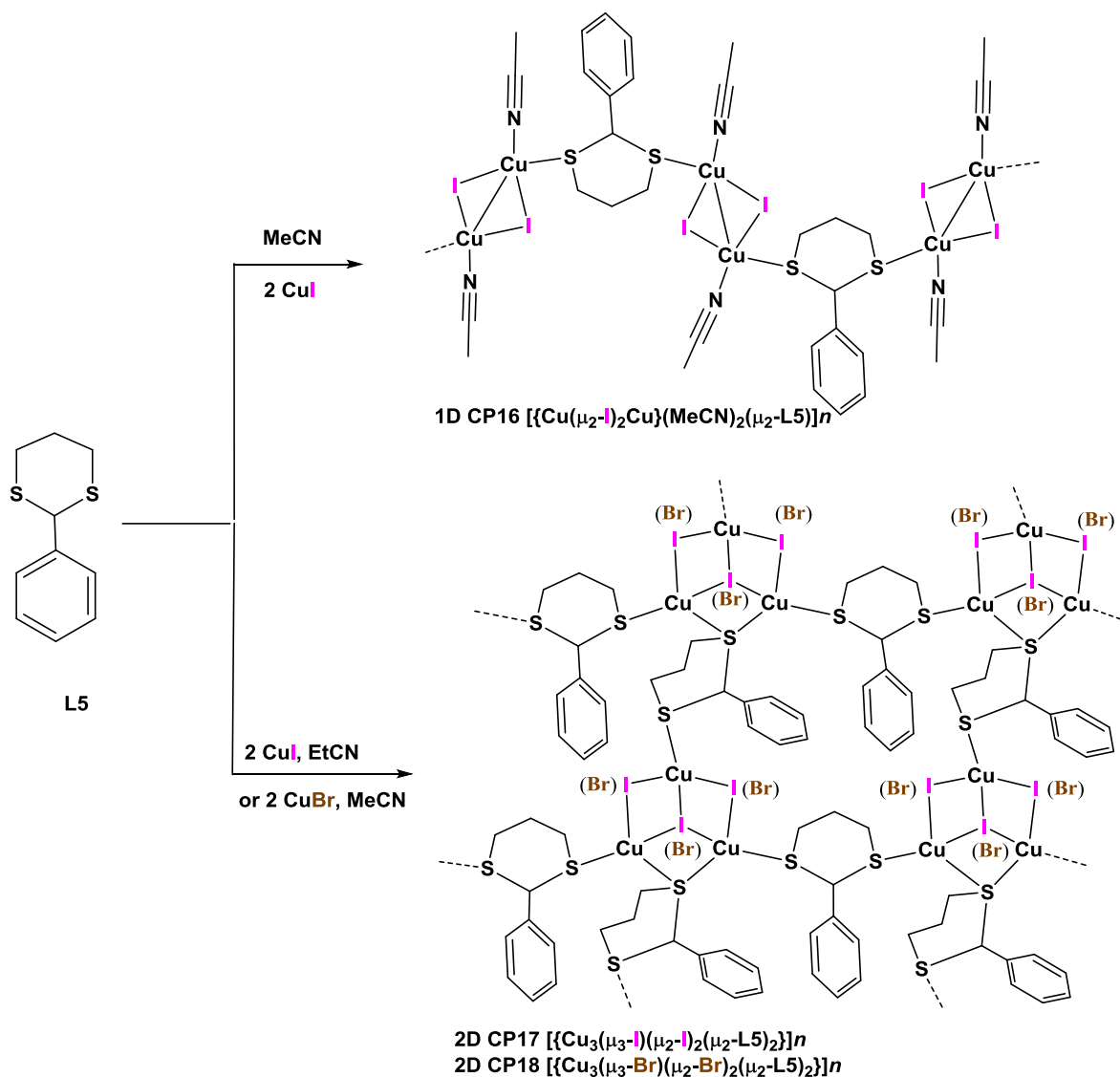
Scheme 6. Synthesis of 1D [\{Cu(\mu_2-I)_2Cu\}(MeCN)_2(\mu_2-L5)]_n CP16 and 2D [\{Cu_3(\mu_3-I)(\mu_2-L5)_2\}]_n CP17 and CP18.
