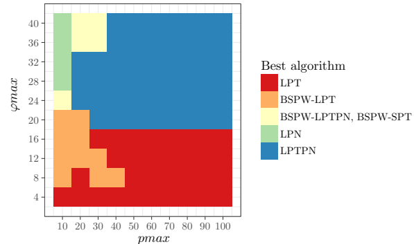
Figure 4: Heat map of the best average makespan performance PERMAK for values of pmax ranging from 10 to 100 and values of \varphi max ranging from 4 to 40.
