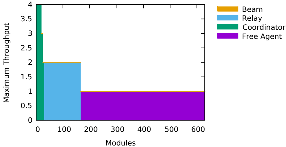
Figure 7: Maximum number of messages sent per module in a single time step for every module during a reconfiguration into a 4-pyramid
