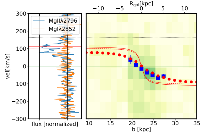
Figure 6. Comparison of galaxy and absorber kinematics at the example of J0145 . Identical plots for all nine galaxy-absorber pairs are available in Fig. D2 of the Supplementary Appendix. The right panel shows the 1D galaxy rotation curve (blue points) obtained from the 2D PVD diagram (shown as background image) on the [OII] doublet (see §6.1). The red points are obtained by reproducing this measurement procedure on the seeing convolved best-fit GalPak 3D model. The solid red line represents the intrinsic GalPak 3D rotation curve along the galaxy major-axis. The dashed red line represents the modeled rotation curve along the line connecting the galaxy and quasar positions on the sky. The lower x-axis represents the distance b from the quasar along this connecting line. The upper x-axis shows the galacto-centric distance along the galaxy’s major axis. In the left panel the MgII \lambda 2796 and MgI \lambda 2852 absorption profiles are shown on the same velocity scale as the galaxy rotation curve. The solid red line in this panel indicates v_{\text{max}} at the observed inclination, which is a continuation of the red curve in the right panel. Similarly, the red dashed line is the continuation of the rotation curve along the galaxy-quasar axis. Further, the black dotted line shows v_{\text{max}} at \text{incl} = 90^\circ and the green line is the systemic redshift as obtained from GalPak 3D ( v = 0 \text{ km s}^{-1} ).
