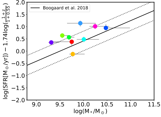
Figure D3. Position of our nine galaxies compared to the main-sequence of star formation (MS). The shown MS (solid line) and its 1\sigma scatter (dotted lines) is from Boogaard et al. (2018). Redshift evolution of the MS ( \text{SFR} \propto (1+z)^{1.74} ) is removed from the plot through the choice of y-axis, which normalises all SFR's to z = 0.55 .
