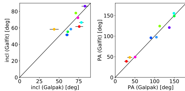
Figure A1. Comparison between GalPak 3D and GALFIT based estimates for the inclination, i , (left) and position angle, PA , (right) for each of the 9 galaxies in our sample. The statistical errors obtained from GalPak 3D are shown as error bars, and are in some cases not visible, as they are smaller than the marker size.
