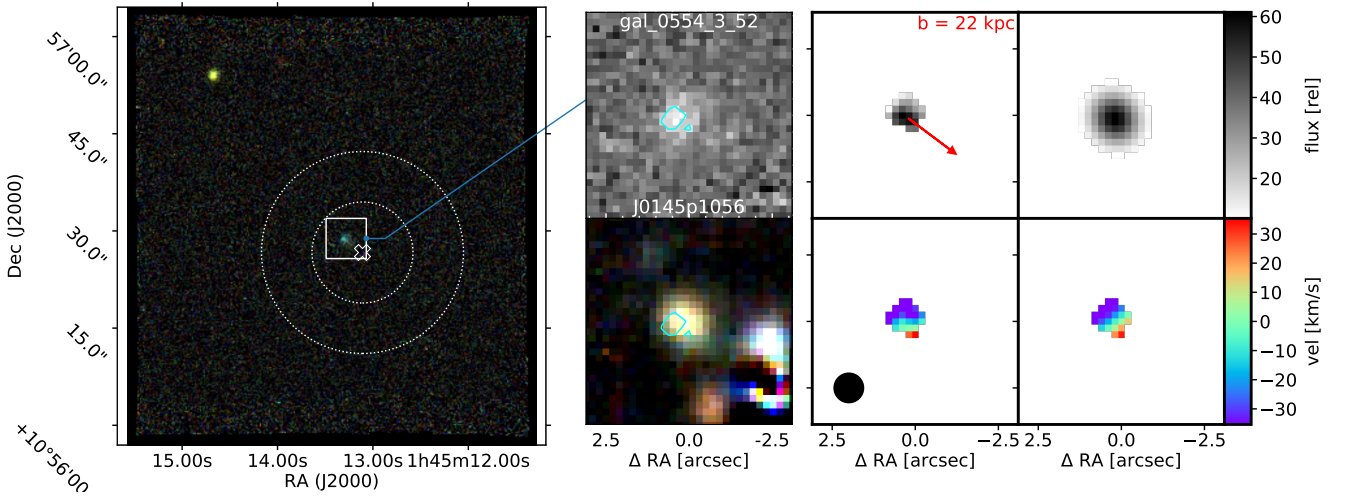
Figure 4. Column 1 (left): Shown is an [\text{OII}] NB image covering \pm 300 \text{ km s}^{-1} around the redshift of the absorber J0145p1056_0554 . More precisely, three slightly different [\text{OII}] NB images were used for each of the three channels of an RGB image. In such an image, emission lines blue-shifted with respect to the absorber redshift appear bluer, while those redshifted will appear redder. The position of the quasar is indicated as a white cross and circles indicate impact parameters corresponding to 50 kpc and 100 kpc. A white box indicates an emission line galaxy associated with the absorber, meaning that the [\text{OII}] emission is in the filter. In the shown example there is only the primary galaxy. The remaining NB excess sources are either due to other emission lines than [\text{OII}] in the NB filter, which means that they are at other redshifts, or residuals from bright objects. Column 2: Top: Simple NB image of the primary galaxy optimised for redshift and width of the [\text{OII}] emission. Overlaid is a contour of this image. Below a colour image is displayed, where pseudo V, R, I broadband images constitute blue, green, and red channels, respectively. The same contour as in the NB image is overlaid. Column 3: Flux (top) and line-of-sight velocity (bottom) maps obtained from direct fitting with CAMEL to the [\text{OII}] cube. More details are given in the text. The filled black circle in the lower left corner indicates the FWHM of the Moffat PSF at the observed wavelength of [\text{OII}] . Column 4: Similar as in column 3, but here the best-fit model flux and velocity maps as obtained from fitting with GalPak 3D are shown. The zero velocity in the velocity maps is taken from the GalPak 3D redshift.
