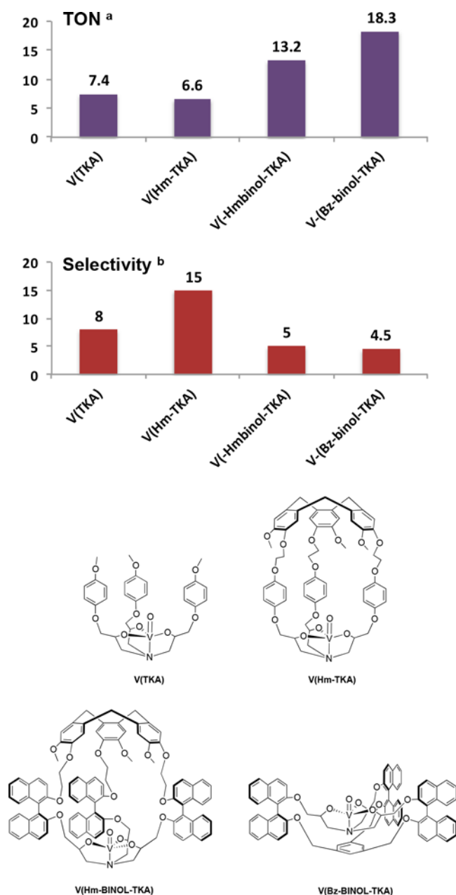
Figure 3. Structures of oxido–vanadium complexes and comparison of their TONs and selectivities to those of the initial oxidation products of methane. Footnote a: moles of (CH 3 OH + CH 3 OOH + HCOOH + HCHO)/moles of catalyst. Footnote b: (CH 3 OH + CH 3 OOH)/(CH 3 OH + CH 3 OOH + HCOOH + HCHO) × 100. For reaction conditions, see Table 1.
