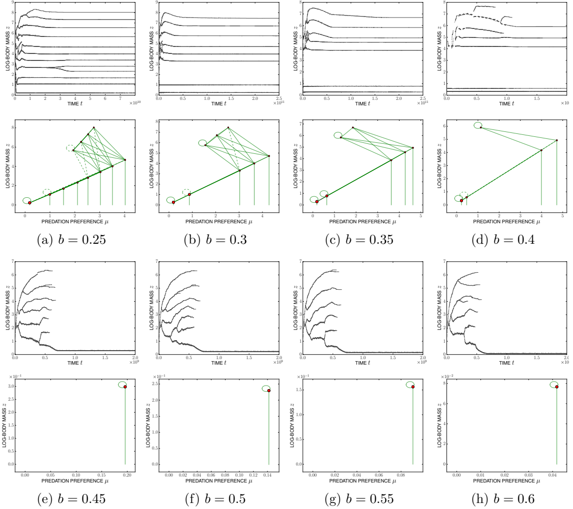
Figure 7: Evolution of the log-mass z (top) and food web at the stationary state (bottom) for b varying from 0.25 to 0.6 with mutation variances \sigma_z = 0.01 > \sigma_\mu = 0.001 , a = 1.2 and \xi_{\max} = 0.75 . Other parameters are given in Table 2.
