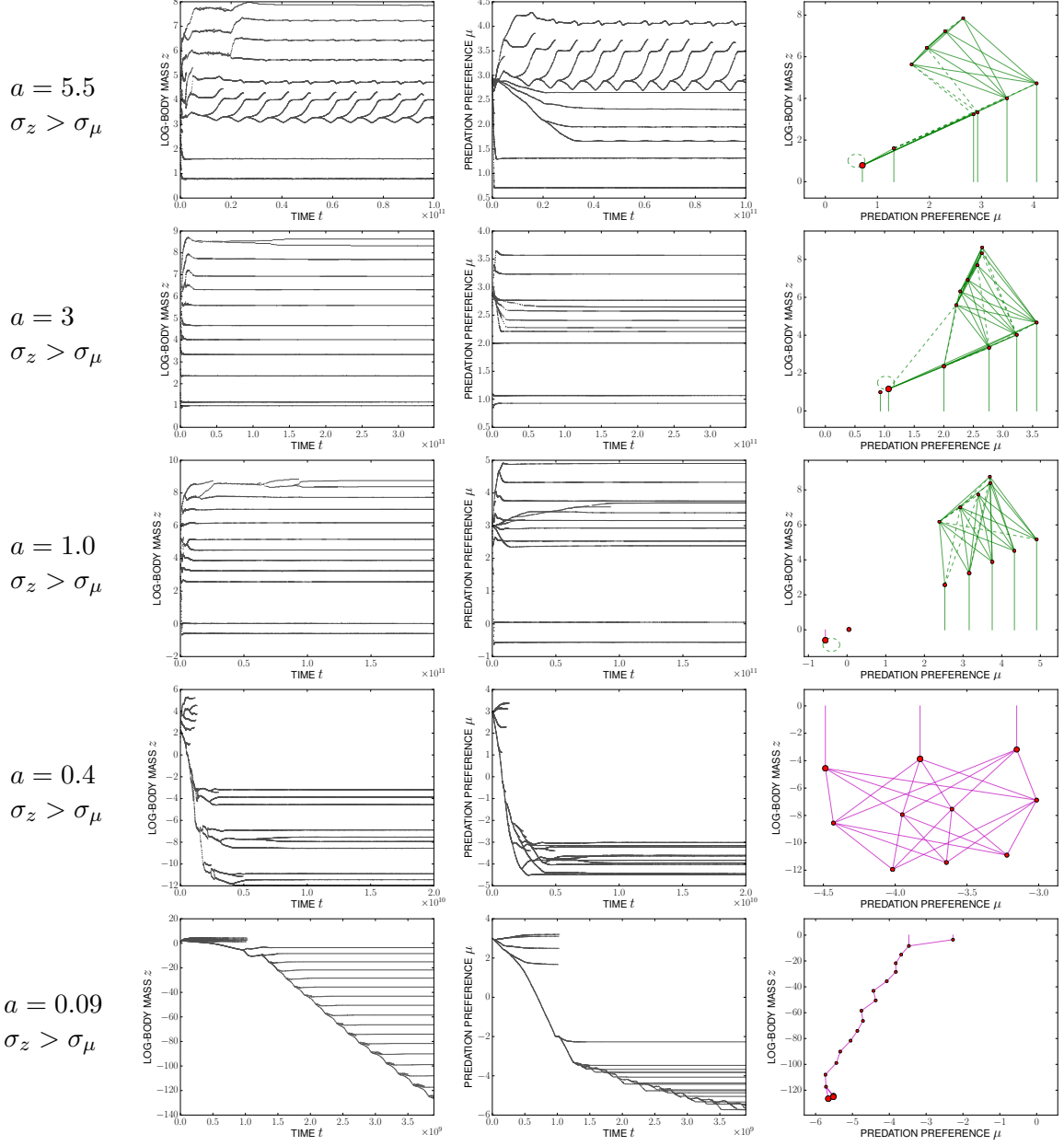
Figure 8: Evolution of the log-mass z (left), evolution of the predation preference \mu (middle) and the final food web (right), for \xi defined by (11) with \xi_{\max} = 0.75 , b = 0.15 , \sigma_z = 0.01 > \sigma_\mu = 0.001 and a varying between 0.09 and 5.5.
