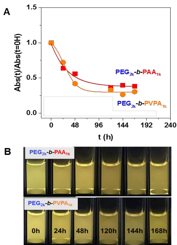
Figure 6. A. Evolution through time of normalized absorbance at 350 nm of ZnO NPs coated by octyl amine or by OA/PEG 2k -b-PAA 1k or OA/PEG 2k -b-PVPA 1k after transfer in water after 0, 24, 48, 120, 144 and 168 hours (normalized absorbance was obtained from Figure S16, see SI for details). B. Corresponding luminescence of these solutions (samples are irradiated at 365 nm)
