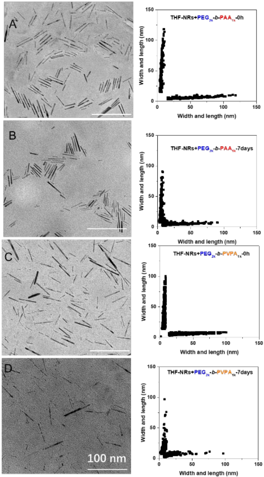
Figure 8. TEM images and corresponding 2D-plots of ZnO nanorods coated by PEG 2k - b -PAA 1k (A and B) or by PEG 2k - b -PVPA 1k (C and D) immediately after modification by the polymer (A and C) or after 7-days aging in THF (B and D).
