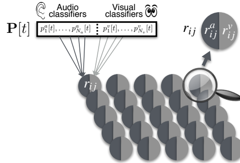
Fig. 7. Illustration of the Multimodal Self-Organizing Map which embeds two sub-networks, each of them being dedicated to coding the information from each modality used to define an object (audition and vision in our case).
