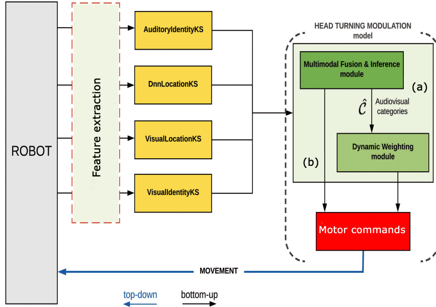
Fig. 5. Schematic architecture of the HTM model and its two main components. (a) The Multimodal Fusion & Inference module, in charge with providing to the DW module corrected audiovisual classes from classification experts outputs. (b) The Dynamic Weighting module, in charge with computing how congruent an audiovisual object actually is, given the environment that it is appearing in. Each of the two modules can trigger head movements separately. The red box depicts the computational component that realizes the combination of the different motor commands and puts them into an order to prioritize one of them, depending on the actual situation
