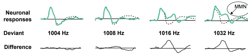
Fig. 3. Mismatch negativity. Upper curve: Neural responses recorded in 80 % of the occurrences of randomly presented sounds of 1000 Hz center frequency ( black dotted lines ), of deviant sounds at different center frequencies in 20 % of the occurrences ( green lines ). Lower curve: Differences of the responses to deviant sounds as compared to the 1000 Hz reference – after Näätänen et al. (2007).
