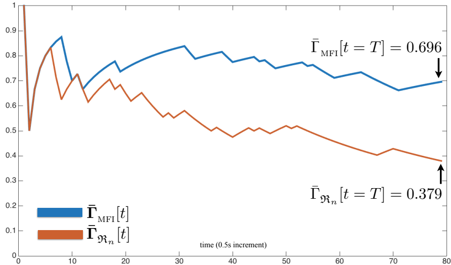
Fig. 12. Average good audiovisual classification rate as a function of time and computed on a rectangular sliding window (that is, at each time frame t , from frame 0 to frame t ) for the MFI ( \bar{\Gamma}_{\text{MFI}} ), ( blue ), and the naive robot ( \bar{\Gamma}_{\mathfrak{R}_n} ), ( red ), that is directly at the classifiers output. The two numbers denote the final results at the end of exploration. Figure adapted from Cohen-Lhyver et al. (2018).
