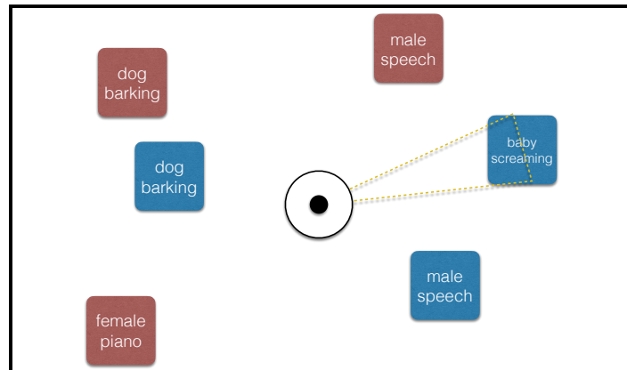
Fig. 10. Illustration of a simulated environment. The environments are populated with various audiovisual sources belonging to a certain audiovisual classes that the robot does not know beforehand. Some of them are emitting sound ( blue ), others are silent, ( red ). The ability of the robot to acquire “correct” knowledge about the semantic content of the scene is assessed on the basis of congruence of the perceived objects, either via the quality of audiovisual fusion or via the quality of head movements triggering or inhibition.
