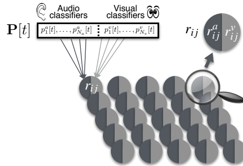
Fig. 7. Illustration of the Multimodal Self-Organizing Map which embeds two subnetworks, each of them being dedicated to coding the information from each modality used to define an object (audition and vision in our case).
