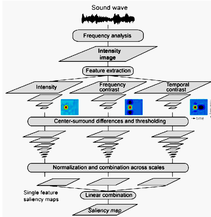
Fig. 4. Building an auditory-saliency map after Kayser et al. (2005), inspired by the work of Koch and Ullman (1985). An acoustic wave is received and then converted into a spectro-temporal representation allowing the extraction of attributes such as intensity, spectral and temporal contrasts. The resulting maps are combined into a comprehensive auditory-saliency map following a normalization step Figure processed
