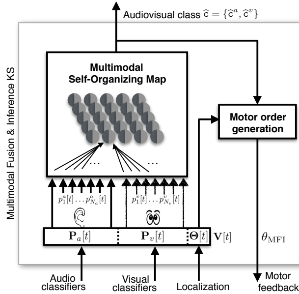
Fig. 6. Multimodal Fusion & Inference module architecture.
