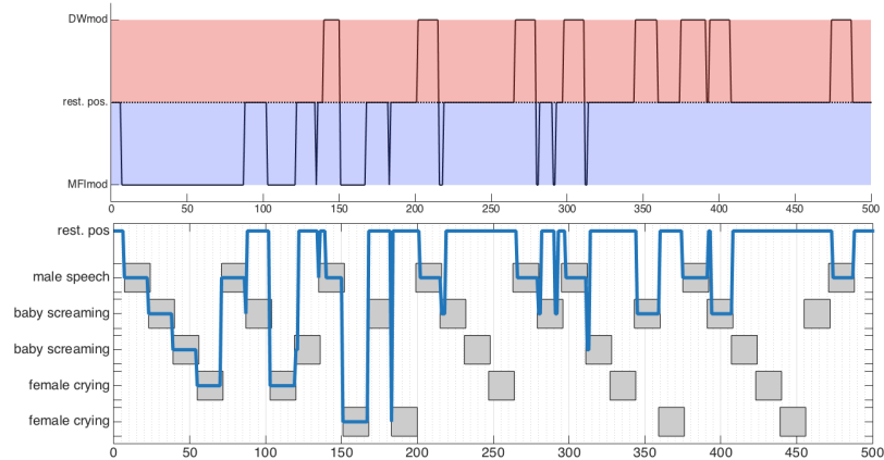
Fig. 9. Three-phase behavior resulting from the combination of the DW and the MFI. Top: Head movements triggered by the DW ( up, red ) or the MFI ( down, blue ). Bottom: Time course of the scenario depicting which and when audiovisual objects are appearing in the environment. The blue line denotes the object to which the robot drives its attention.
