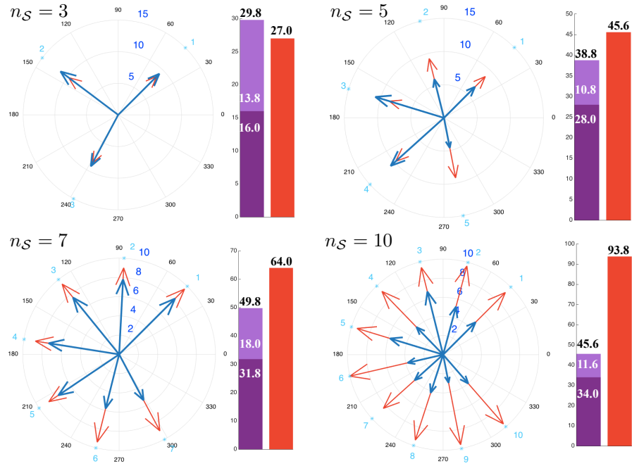
Fig. 11. Number of head movements generated in multisource scenarios. Movements generated by the HTM, ( blue ), and by the naive robot, ( red ). The arrows point to the positions of audiovisual sources, their length representing the number of movements toward the considered source. The histograms depict the total sum of generated movements, by the MFI, ( dark purple ), by the DW, ( light purple ), and by the naive robot, ( red ). The ( white ) numbers correspond to the number of movements by module, averaged over five trials, and their sum, ( black ).
