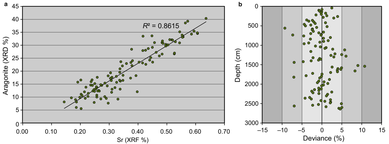
FIGURE 2 (a) Correlation between strontium, as measured in quantitative X-ray fluorescence (XRF), and aragonite, as measured by powder X-ray diffraction (XRD). A single outlying point (from 980 cm depth in the core) removed. R^2 value of the correlation = 0.8615. (b) Deviation of aragonite content derived from XRF Sr data from quantitative XRD measurements, showing <10% variance overall, indicating that XRF data are a reasonable approximation of aragonite content
