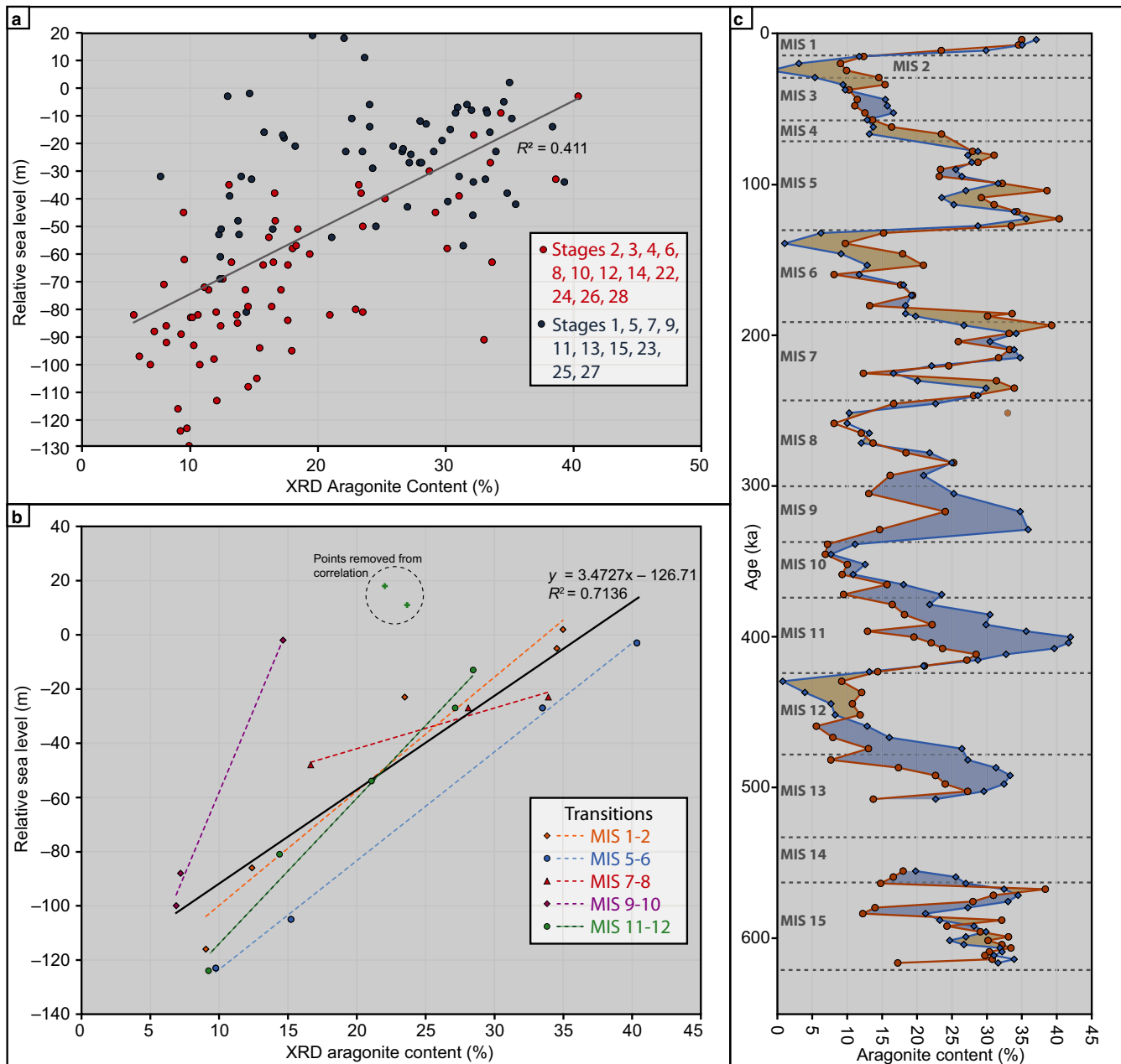
FIGURE 7 (a) Cross-plot of sea-level and aragonite content as determined from X-ray diffraction (XRD) analysis. All data points shown. Stage boundaries from Cohen and Gibbard (2008). (b) Cross-plot of aragonite and sea-level during selected glacial–interglacial transitions, shown in legend. (c) Plot of actual aragonite content (orange line, derived from XRD) and aragonite content as predicted by the relationship calculated in Figure 4b (blue line). Shading indicates the line with greater values
