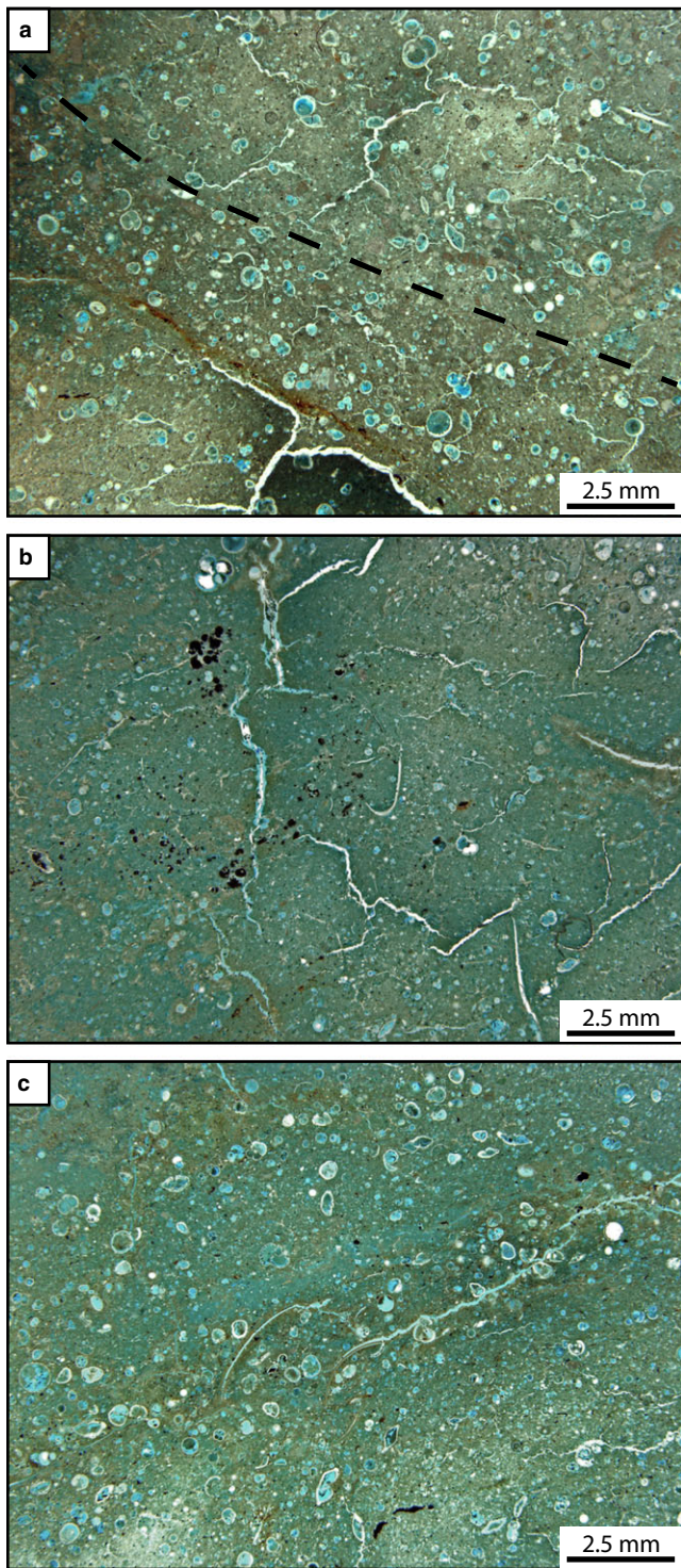
FIGURE 6 Thin sections of sediments adjacent to proposed unconformities. All sections vacuum impregnated with blue epoxy. (a) Section centred around 1,785 cm depth (upper unconformity) showing contact between two sediment types marked by dashed line. (b) Sediment just above lower unconformity, 2,182 cm depth, showing sediment dominated by fine-grained mudstone with few planktonic foraminifers. (c) Sediment just below lower unconformity, showing increase in foraminifer content relative to b). Same scale on all images
