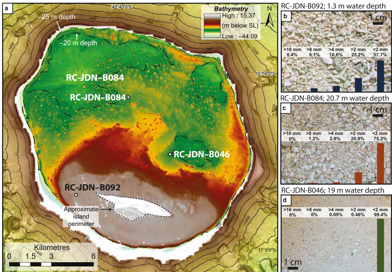
FIGURE 3 (a) High-resolution LIDAR bathymetry and topography of Juan de Nova island and platform top, and swath bathymetry around the seamount. Location of sediment samples in b–d labelled. (b–d) Representative sediment samples and grain-size data from the platform top
