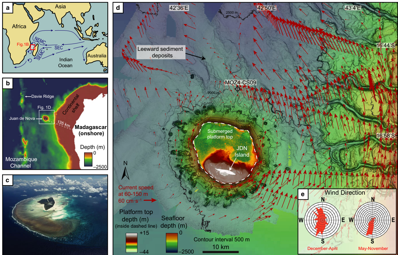
FIGURE 1 Location and background of Juan de Nova platform. (a) Location of study area relative to large-scale currents in the Indian Ocean. Ocean circulation data from Schott et al. (2009). SEC: South Equatorial Current; NEMC: Northeast Madagascar Current; SEMC: Southeast Madagascar Current. (b) Bathymetry of the northeastern Mozambique Channel, showing isolation of Juan de Nova platform from Madagascar shelf. (c) Aerial photo of subaerial and shallow marine portions of Juan de Nova. Modified from Jorry et al. (2016), picture from French Southern and Antarctic Lands (TAAF). (d) Detailed bathymetry of platform top (Lidar data from the Litto3D program), flanks and adjacent sea floor (PTOLEMEE cruise; Jorry, 2014), with superimposed shallow current data (computed from ADCP data, PTOLEMEE cruise; Jorry, 2014). (e) Wind data (490 measurements December–April, 764 measurements May–December; Météo France, 2017) collected from a weather station on the island
