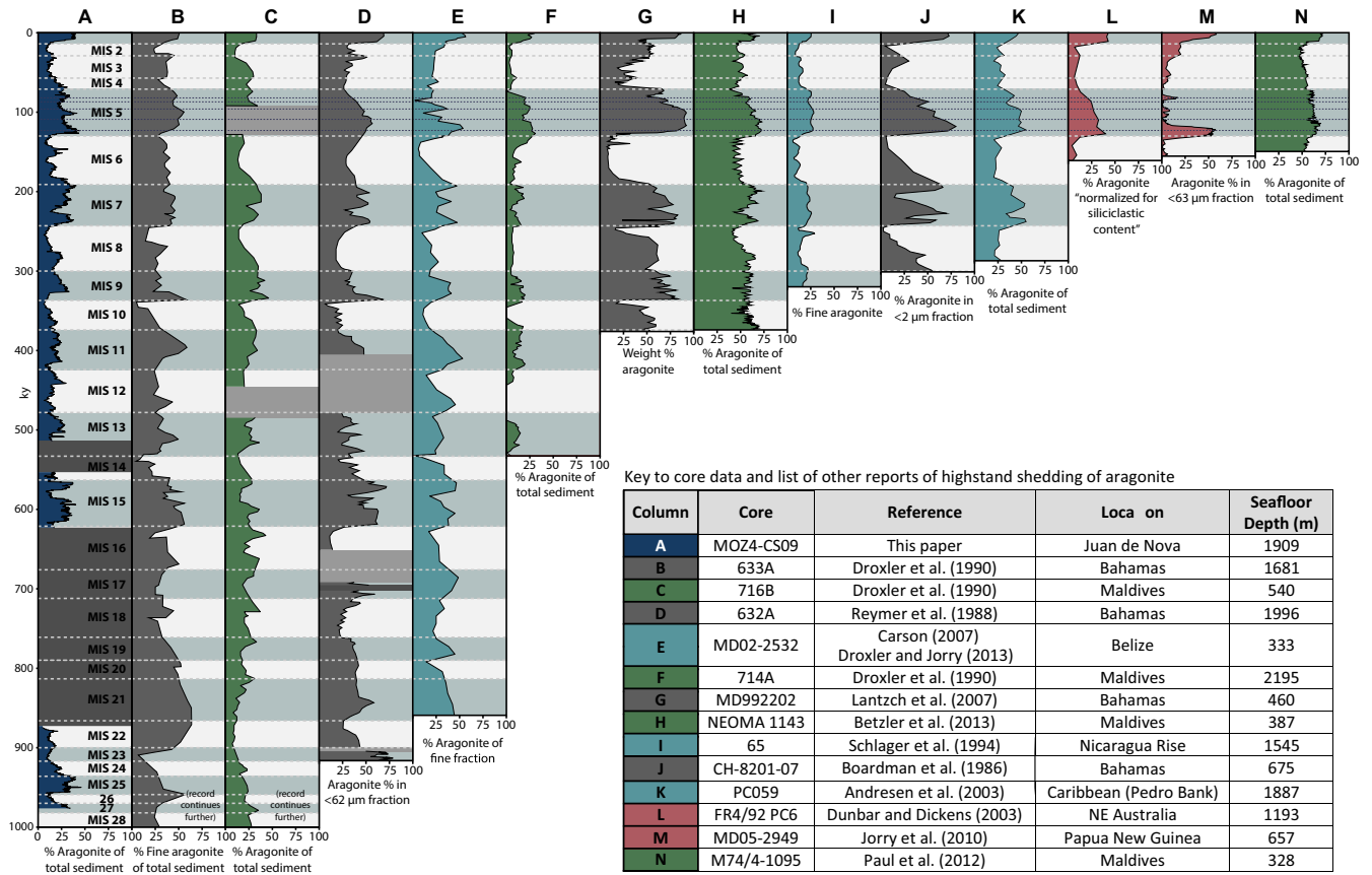
FIGURE 9 Comparison of the aragonite records of 13 global localities with that of Juan de Nova. Aragonite curves redrafted from publications listed in table, except for E and M, where only aragonite mass accumulation rates have been published and aragonite content was back-calculated. Each record is presented on its originally published age model; conversion of original low-resolution raster data into the form shown here may introduce additional error. This compilation should therefore not be used to analyse the exact timing and magnitude of aragonite content changes in detail, but is instead meant to illustrate larger scale trends
