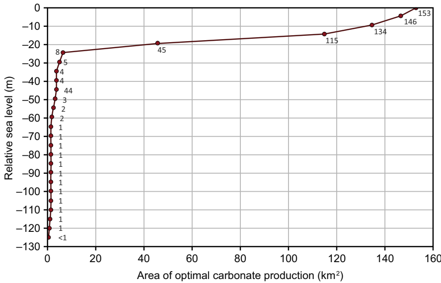
FIGURE 8 Relationship between sea-level and the area available for optimal carbonate productivity, defined here as water depths of 20 m or less. Values rounded to nearest km 2
