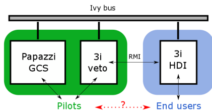
Figure 4: Architecture of the 3i UAS HDI
