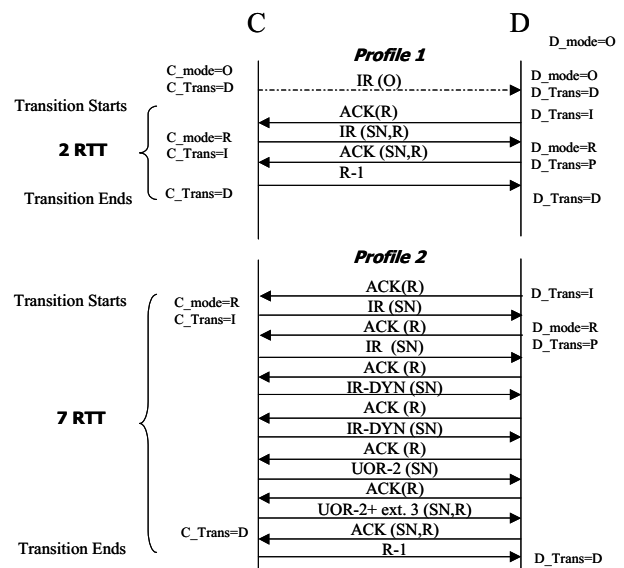
Figure 5. Mode Transition in Profile 1 and Profile 2 based profiles.
