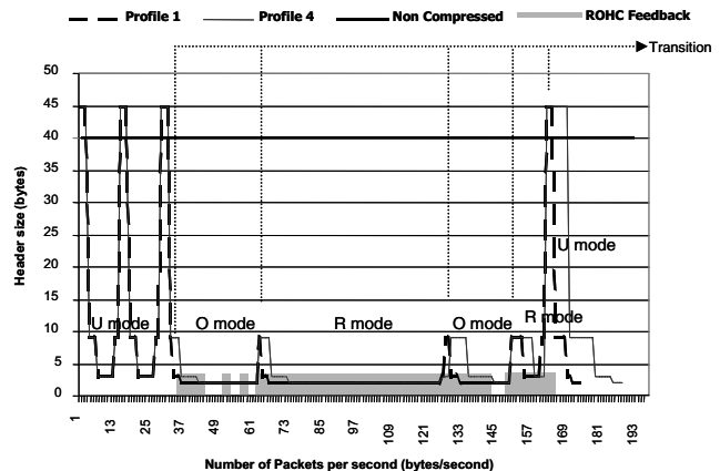
Figure 2. ROHC compression for Profile 1 and 4 without error. The compressor is using the three Operation Modes (U, O, R), the five Transition Modes and the use of feedback in the bi-directional modes.
