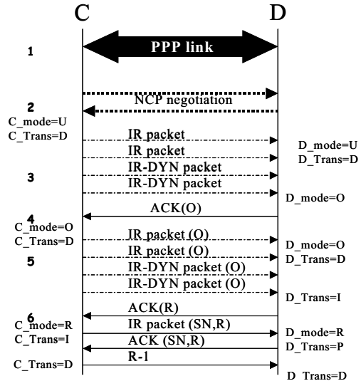
Figure 1. ROHC Information Flow. After the PPP channel is opened the NCP negotiated able the ROHC compression. Two variables are kept in each side Transition and Mode.
