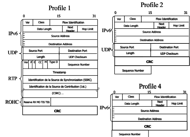
Figure 4. The computing of CRC for ROHC profiles
