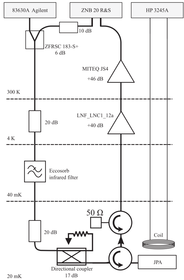
FIG. 6. Experimental setup.
