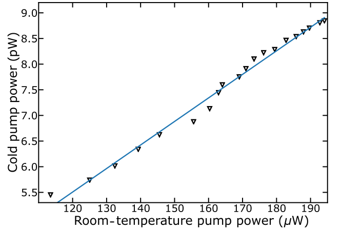
FIG. 9. Power at the input of the JPA versus room temperature power.
