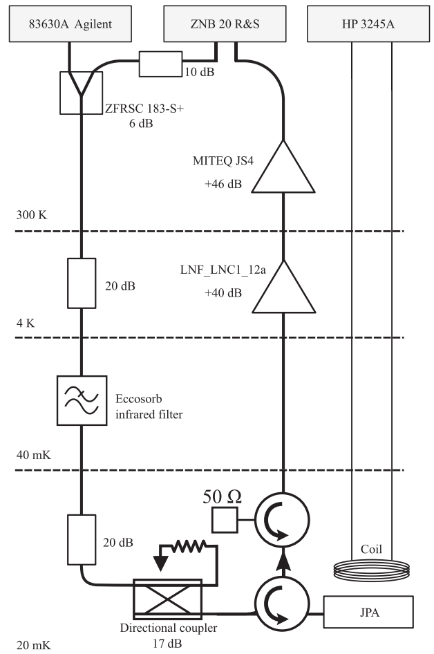
FIG. 6. Experimental setup.
