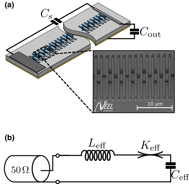
FIG. 1. (a) Sketch of the JPA based on an array of 80 SQUIDs. We highlight the capacitance C_{\text{out}} between the last superconducting pad and the ground and the parasitic shunt capacitance C_s between the input/output pad and the last superconducting pad. Enlargement: SEM image of seven identical SQUIDs, where a single junction has an area of 10.7 \times 0.370 \mu\text{m} . (b) Effective LC series nonlinear resonator.
