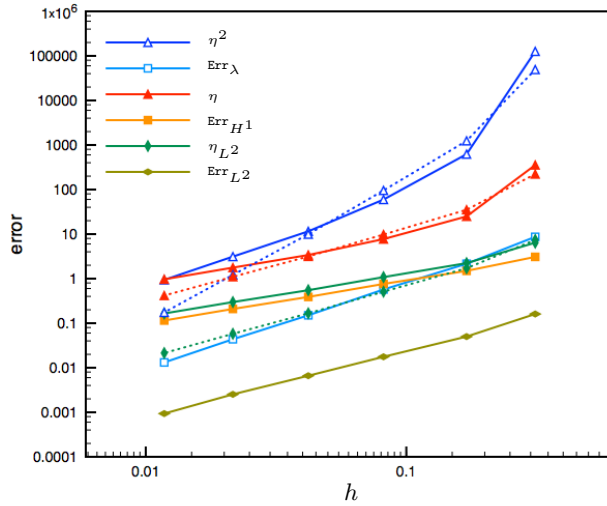
Figure 2: Convergence of various measures of the error and their upper bounds for finite elements and the unit square with m = 2, M = 3 (top) and for the L-shaped domain with m = 3, M = 5 (bottom). The dotted lines provide the estimators using Case II with \delta = \frac{2}{3} and the empirical choice C_S = C_I = 1 .
