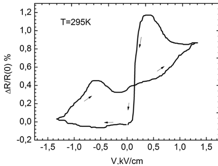
Figure 6: Dependence of the resistance of the LBMO film on the electrical voltage applied to the substrate
