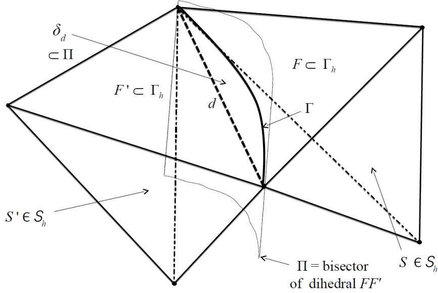
Figure 2: Plane skin \delta_d for two tetrahedra S, S' having faces F, F' \subset \Gamma_h with F \cap F' = \text{edge } d
