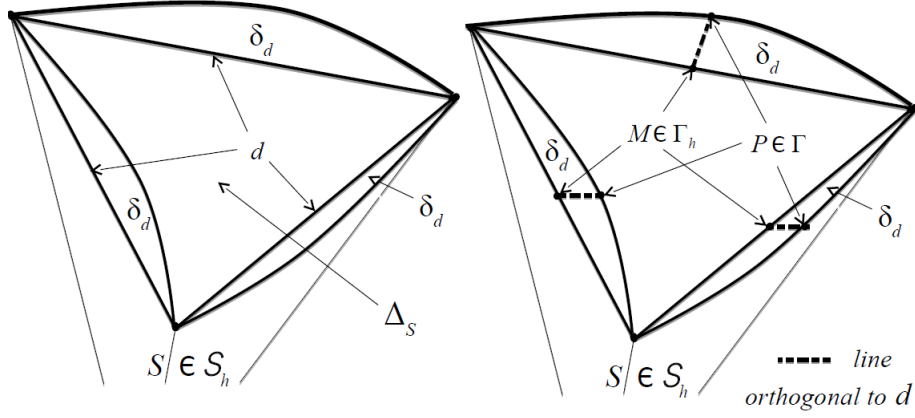
Figure 3: Set \Delta_S for a tetrahedron S \in \mathcal{S}_h and its nodes (right) P \in \Gamma associated with M \in \Gamma_h
