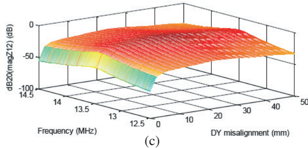
Figure 9. Level of simulated \text{dB}_{20}(\text{mag}Z_{12}) versus the frequency band and the DY misalignment for d = 10 mm in VM mode. (a) A_{\text{reader}} in center. (b) B_{\text{reader}} in center. (c) E_{\text{reader}} in center.
