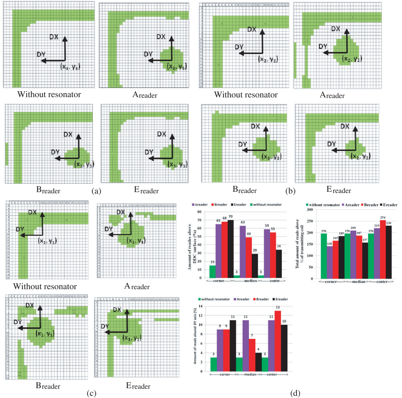
Figure 7. Results of RFID tag detection in VM, for coil A_{\text{reader}} , B_{\text{reader}} and E_{\text{reader}} (colored cells), in function of DX and DY (lateral misalignments) versus the DDC position (corner, median, center) at 30 mm coaxial distance and 13.56 MHz. (a) DDC in the center position ( x_3 = 0, y_3 = 0 ) in Fig. 2(c). (b) DDC in the median position ( x_2 = -7.5 \text{ cm}, y_2 = -3.75 \text{ cm} ) in Fig. 2(c). (c) DDC in the corner position ( x_1 = -15 \text{ cm}, y_1 = -7.5 \text{ cm} ) in Fig. 2(c). (d) Results of RFID tag detection cases above DDC surface, above a quarter of the reader surface, and along the y axis.
