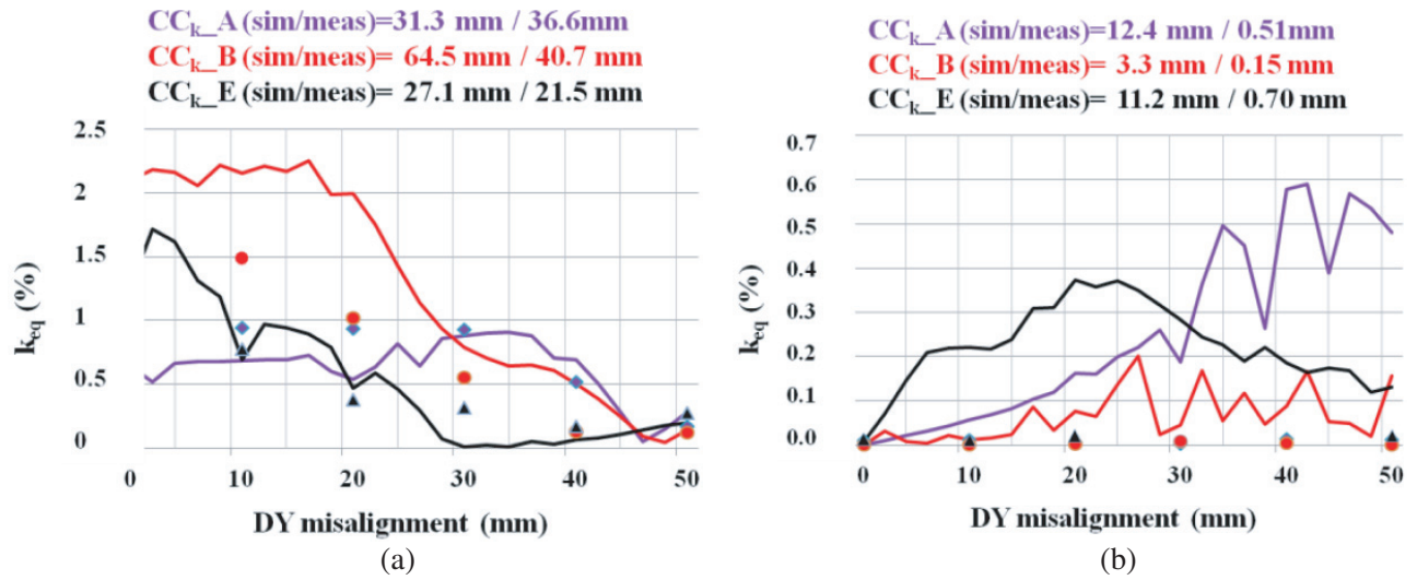
Figure 5. Simulated (solid line) and measured (dot) coupling coefficient versus DY misalignment for d = 10 mm at 13.56 MHz. (a) For HM mode, (b) for VM mode.
