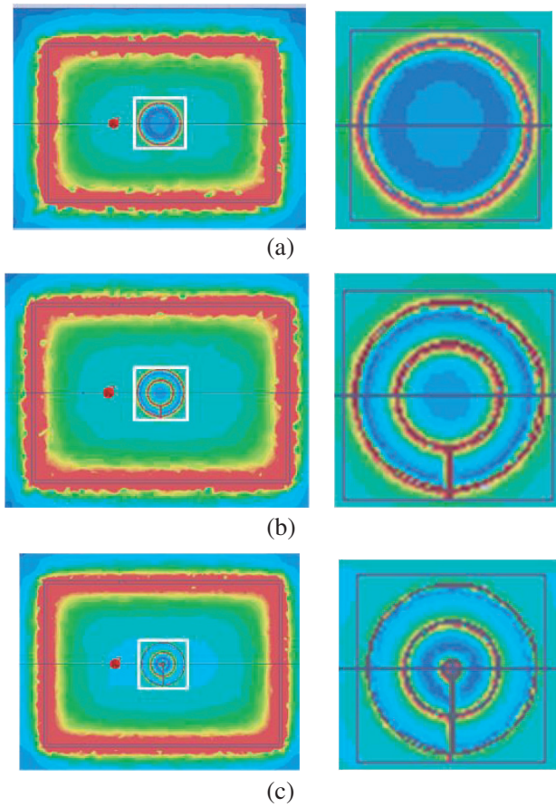
Figure 6. H-field relative magnitude and distribution in (Y0Z) plane with same color scale, in left side, onto the reader coil and in right side, above the resonator. (a) A_{reader} , (b) B_{reader} , (c) E_{reader} .
