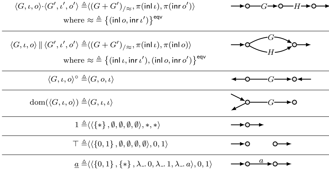
Fig. 6: The algebra of 2p-graphs.
