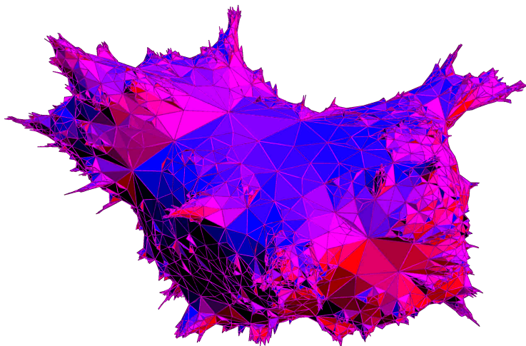
FIGURE 3. A random bipolar orientation of an triangulation with 5000 faces (© Jérémie Bettinelli). The orientations of the edges are not shown.
