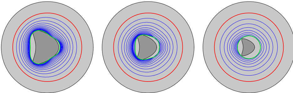
FIG. 5.4. Iterates (in blue) and the final reconstructions (in green) for different scalings of a kite shaped void with 1% noise.
