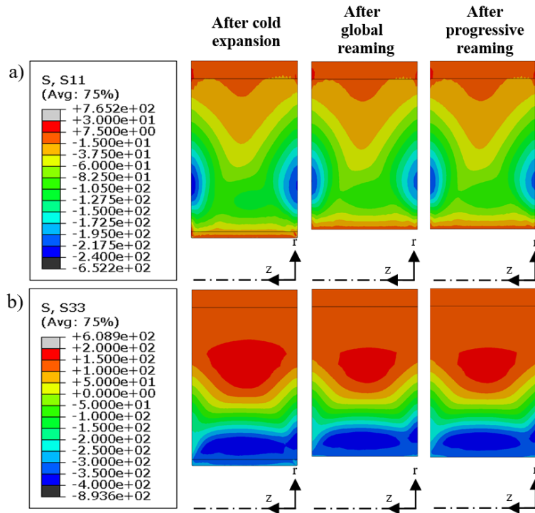
Fig. 5. Radial (a) and circumferential (b) stress states obtained in the part at the end of the cold expansion (1 st column), global (2 nd column) and progressive (3 rd column) reaming simulations
