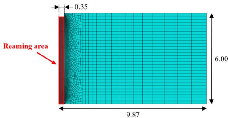
Fig. 4. Representation of the reaming area and the deactivated elements in the first calculation step for the progressive reaming (Dimensions in mm)
