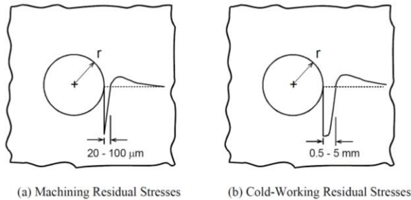
Fig. 1. Residual stress induced by machining (a) and cold expansion process (b) in a 2024-T3 aluminum alloy part [11]
