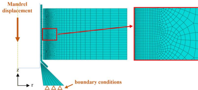
Fig. 3. Mesh of the numerical model
