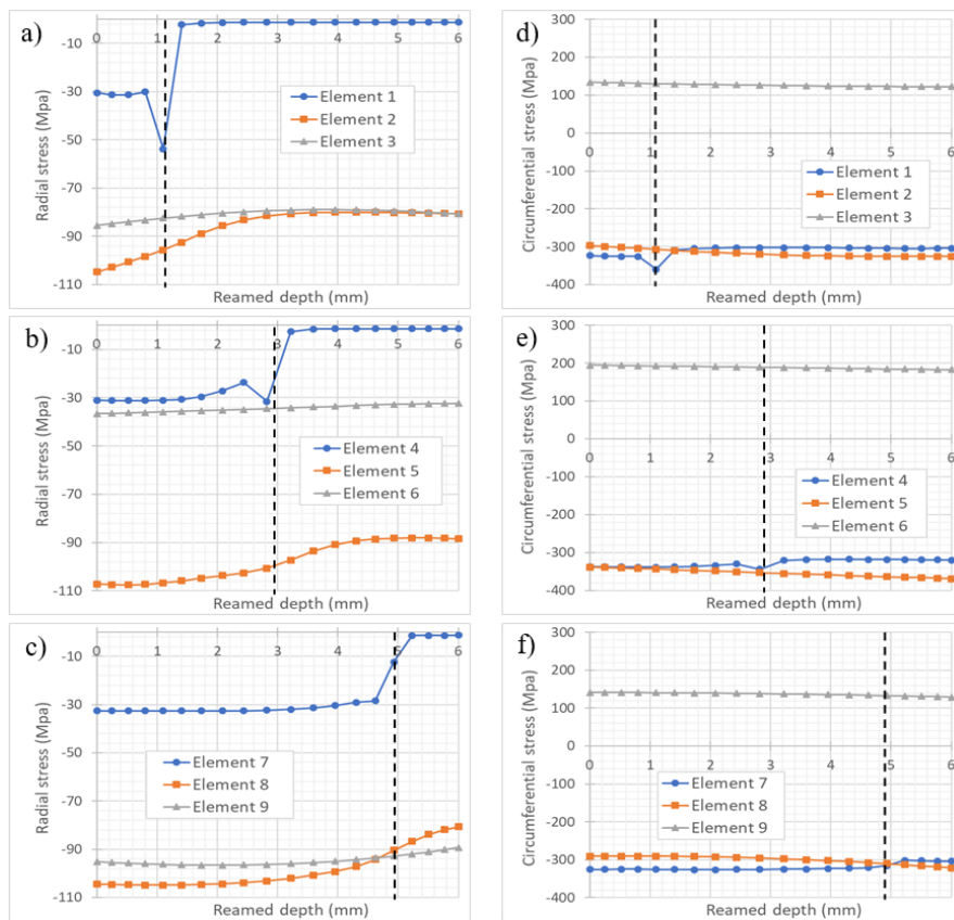
Fig. 8. Evolution of radial (a,b,c) and circumferential (d,e,f) residual stresses during progressive reaming simulation
