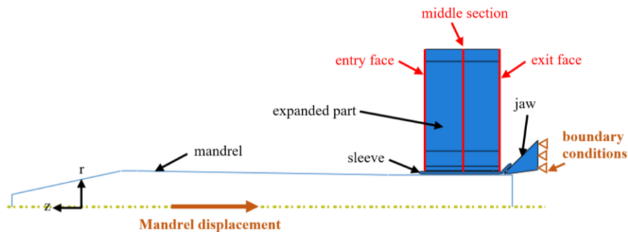
Fig. 2. Finite element model of the cold expansion process.
