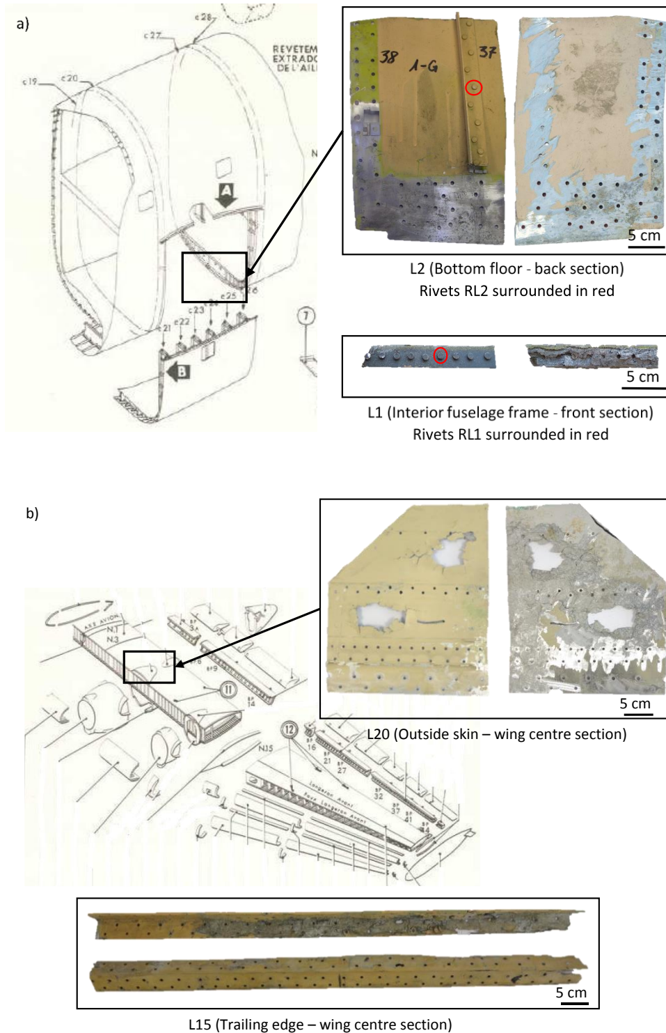
Figure 1. Photographs of collected parts (front and back side) from Breguet 765 airplane with localization on original plans (Breguet n.d.); a) Plate L2 (2 mm thick) with RL2 rivets (5 mm diameter) and profile L1 with RL1 rivets (4 mm diameter), b) Plate L20 (3 mm thick) and profile L15 (4 mm thick); c) Plate L8 (1.6 mm thick) and bracket L9 (5 mm thick).
