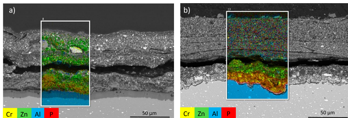
Figure 1. Coating detected in L9 (back side) and L15 (front side) with SEM: backscattering image and EDS maps. Only Zn, P, Cr and Al are shown. In blue: Al-alloy, green: zinc, yellow: chrome and red: phosphorus.
