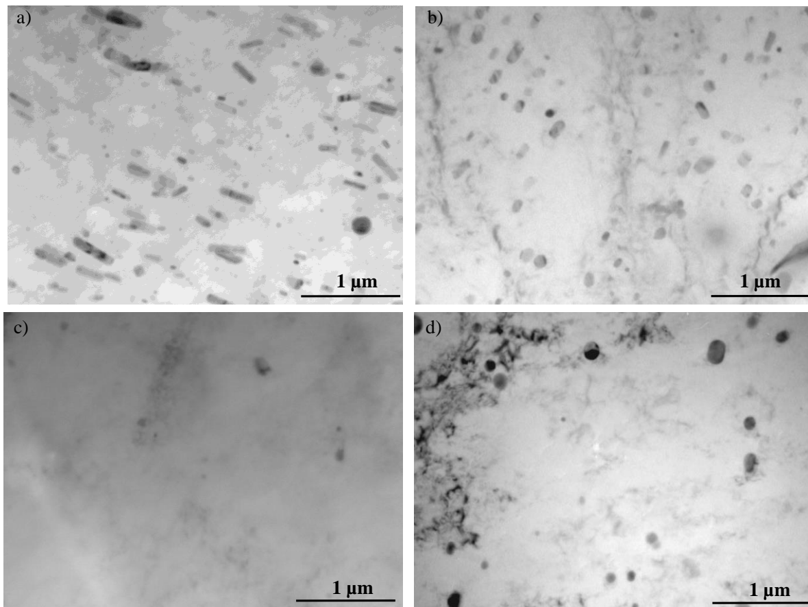
Figure 3. Observations by TEM of dispersoids in top row (bright field observation): a) plate L2 (A-U4G1), b) plate L8 (A-U4G), c) rivet RL1 (A-U3G) and d) rivet RL2 (A-U4G).
