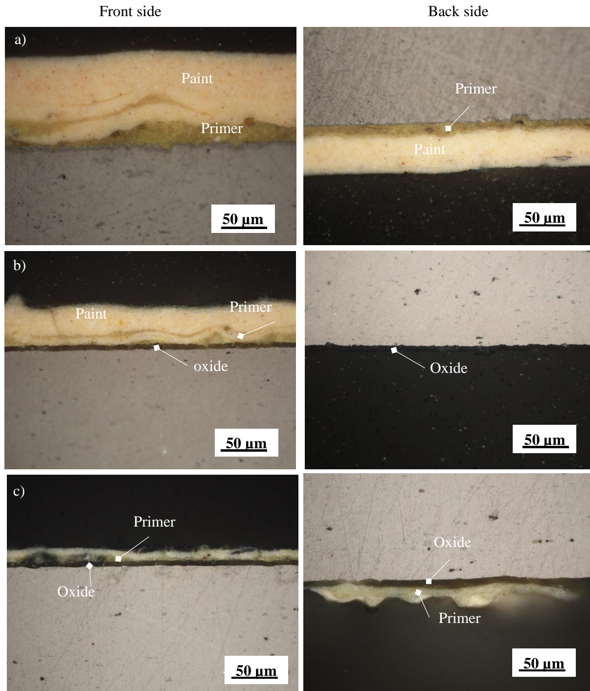
Figure 4. Optical microscope images (dark field mode) of protective coatings for both sides: a) L2, b) L8, c) L20, d): L9, e) L15, f) RL1, g) RL2. For L9, the front side was completely corroded and the coating no longer existed
