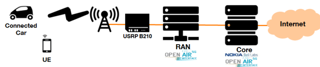
Fig. 1: Network architecture
