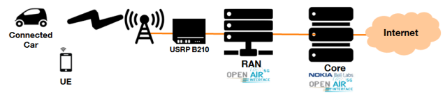
Fig. 1: Network architecture
