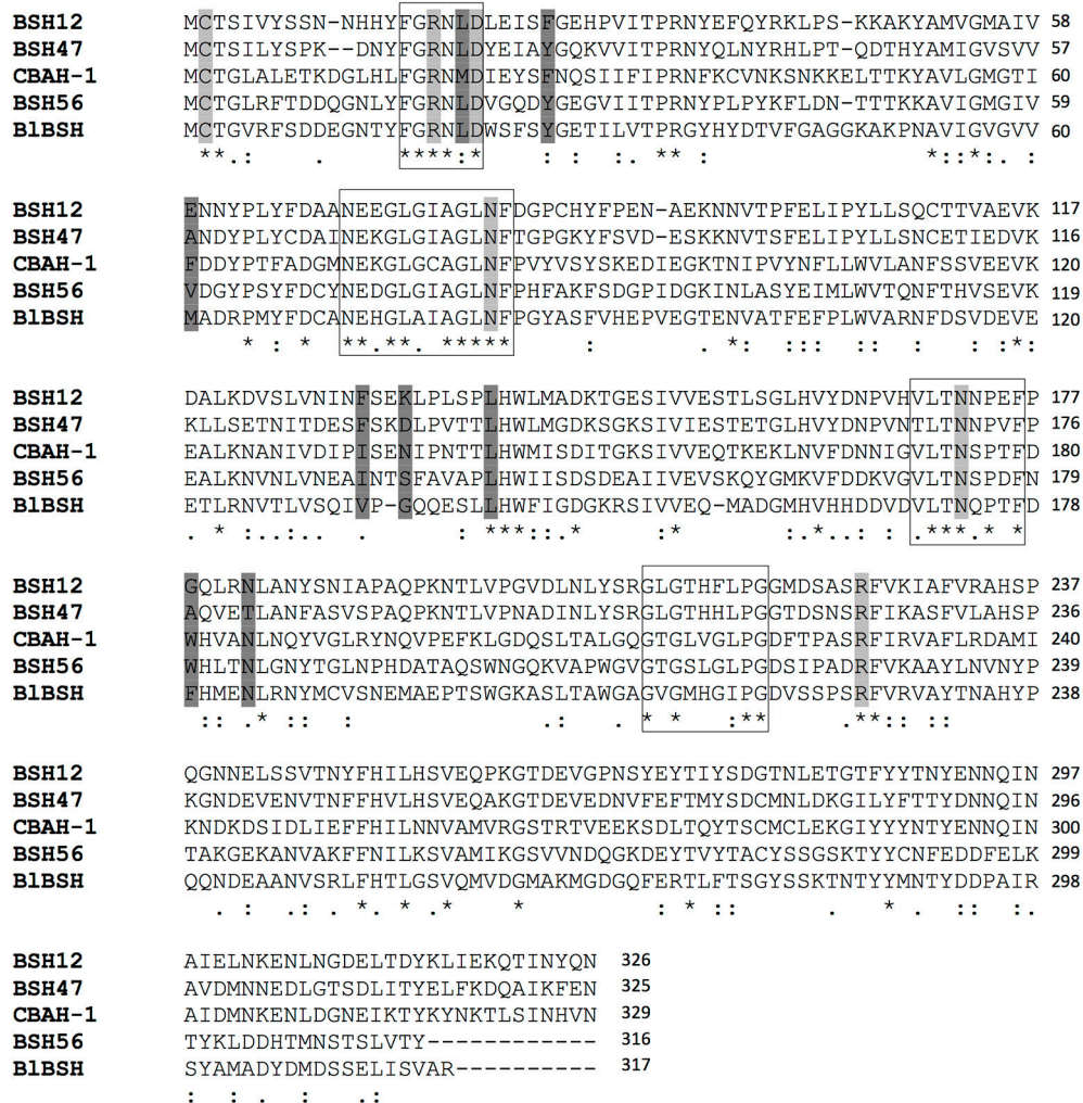
FIGURE 1 | L. johnsonii La1 BSH possess conserved key amino acids in their predicted active sites. Multiple sequence alignments of BSH were performed with the ClustalO program ( http://www.ebi.ac.uk/Tools/msa/clustalo/ ) using GONNET 250 matrix. An "*" (asterisk) indicates positions of fully conserved residues in all five sequences; a ":" (colon) indicates conservation of amino acid with strongly similar chemical properties (Gonnet PAM 250 matrix score > 0.5); a "." indicates conservation of amino acid with similar chemical properties (Gonnet PAM 250 matrix score ≤ 0.5). Residues highlighted in light gray correspond to the predicted key active site amino acids, based on the 3D structures of BSHs from both C. perfringens (CBAH-1, PDB: 2BJF) (Rossocha et al., 2005) and B. longum (B1BSH, PDB: 2RF8) (Kumar et al., 2006). Residues highlighted in dark gray indicate amino acids putatively involved in substrate binding based on CBAH-1 3D structure (Rossocha et al., 2005; Ridlon et al., 2006). Boxes indicate conserved signatures, i.e., 16 FGRNLD, 72 NEXGLXXAGLN, 170 VXXLTNXPX, and 213 GXGXGXGPGD (CBAH-1 numbering).
