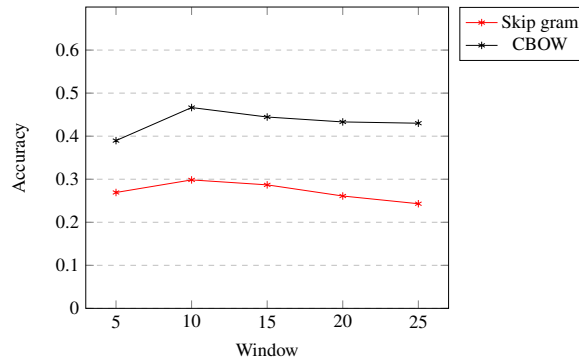
Fig. 3. Accuracy variations according to window size for CBOW and Skip-gram models with fixed dimensional vector model (size=300)
