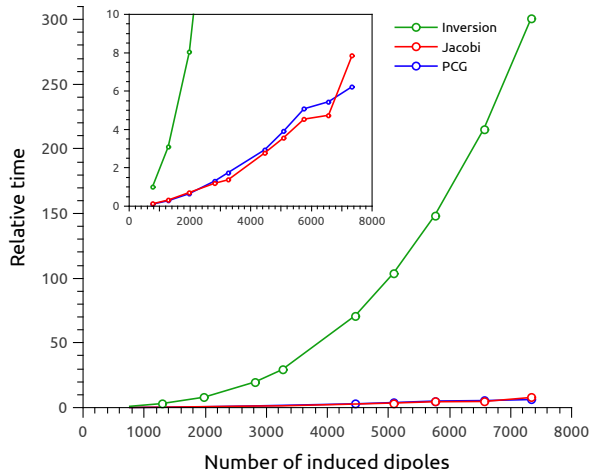
Figure 1: Relative times needed to solve for the induced dipoles, using different methods. Green line: inversion; Red line: Jacobi Iterations; Blue line: Preconditioned Conjugate Gradient. The times are cumulative and refer to the sum of all SCF cycles until convergence is reached. The number of SCF cycles considered is the average one across the various structures considered. The values have been normalized for comparison with respect to the time required to solve the smallest polarisation problem (7 Å polarization radius, 765 induced dipoles) with the inversion procedure.
