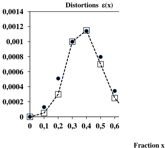
Fig. 4: Observed (square) and calculated (round) distortion functions \varepsilon_{obs}(x) and Y_\varepsilon(x) = \varepsilon_{calc}(x) . Parameters: \varepsilon_{AA} = \varepsilon_{BB} = 0 ; \varepsilon_{AB} = 0.005 ; x_{AA} = 0 ; x_{BB} = 1 ; x_{AB} = 0.35 ; k_{AB} = 20 .
