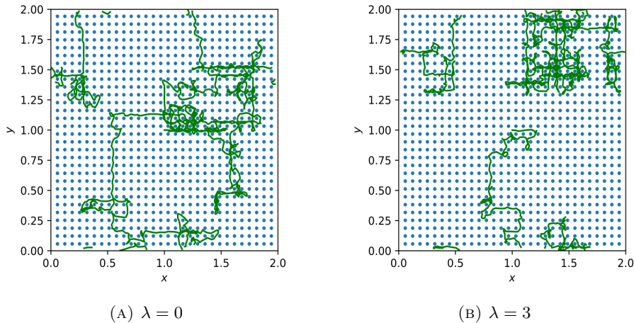
FIGURE 10. Particle’s trajectories for N = 900 obstacles. Paramters: \alpha = 0 , \beta = 0 , \sigma = 1 , \lambda = 0 (10a) and \lambda = 3 (10b).
