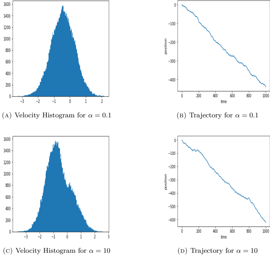
FIGURE 7. Histogram for the velocity V solution of Equation (6) (7a,7c) and cell trajectory (7b,7d) for h = 0.5 , \lambda = 1 , \gamma = c = \sigma = 1 , \beta = 0.1 , \alpha = 0.1 (7a,7b) and \alpha = 10 (7c,7d).
