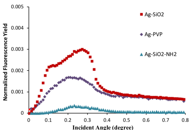
Figure 4: Observed LP-XSW Ag L \alpha fluorescence yield (FY) profiles for different NPs' coating: Ag-SiO 2 -NH 2 (triangles), Ag-SiO 2 (squares) and Ag-PVP (diamonds) exposed to solution/ S. oneidensis MR-1 biofilm/ \alpha -Al 2 O 3 (1-102) interface after (a) 3 hours (open symbols) and (b) 24 hours (closed symbols).
