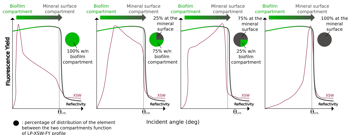
Figure 2: Schematic diagram showing LP-XSW-FY profiles that might be observed as a function of different elemental spatial distributions. This figure is adapted from Templeton et al., 2009 40 .
