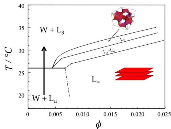
Figure 1. Partial phase diagram, at high water content, of the water- C_{10}E_3 system adapted from 15 . Here, L_\alpha refers to lamellar phase, L_3 to a “sponge” ( L_3 ) phase and W to a solution phase. \phi denotes the surfactant concentration. The horizontal line at 26 °C corresponds to a three phase line, W + L_\alpha + L_3 . The vertical arrow illustrates a typical temperature jump.
