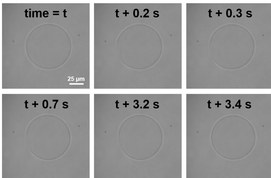
Figure 4: Membrane pore captured for a GUV under irradiation (light intensity = I) with 4 μM DO15, showing a pore from t+0.2 s of irradiation, after the end of the strong shape fluctuations period.
