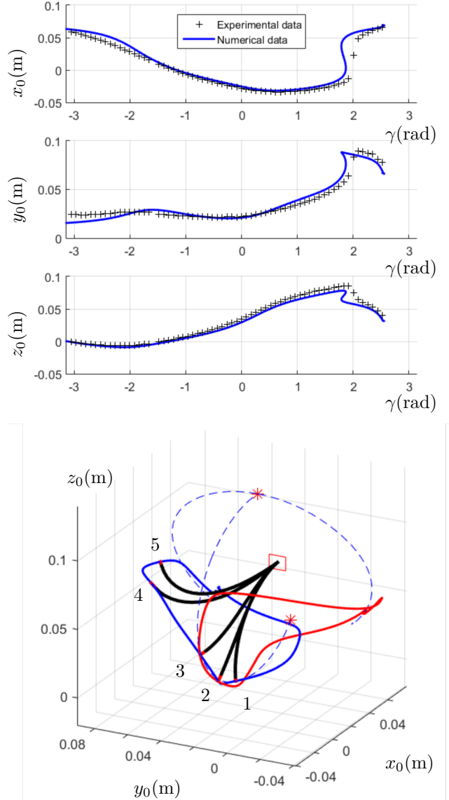
Figure 8: Experimental confrontation for \mathbf{B}_r rotating in (x_0, z_0) plane. Top: Comparison between numerical and experimental results in term of tip coordinate in \mathcal{R}_0 . Numerical results are represented in blue line and experimental tip position coordinates with black crosses. Bottom: Comparison of the robot tip trajectory computed with homogeneous (dotted line) and inhomogeneous field (plain line). Branches are computed for two proximal position, \mathbf{p}_0 in blue and \mathbf{p}_{0b} in red.
