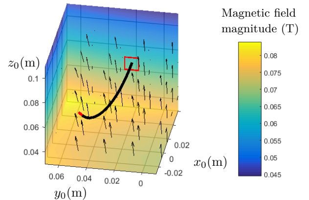
Figure 1: Representation of a one-magnet m-CR controlled with the CardioMag MNS [1]. A desired magnetic field of magnitude 0.08T is generated in [0, 0, 0] . The m-CR is clamped at the center of the red square.
