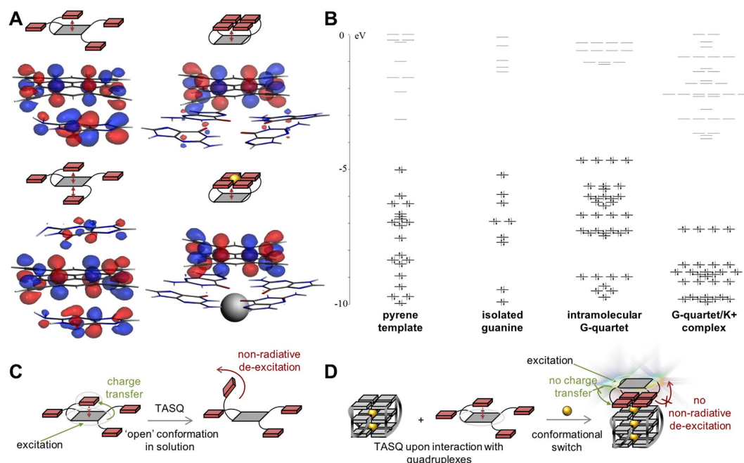
Figure 3. Molecular orbital analyses of the conformations of PyroTASQ. (A) Determination of the HOMO of two simplified 'open' models (left) and two simplified 'closed' models (right). (B) Molecular orbital levels of pyrene, guanine, G-quartet and G-quartet/K + complex. (C, D) Schematic representation of the newly postulated mechanism that explains the turn-on fluorescence properties, that is, the smart nature of PyroTASQ.
