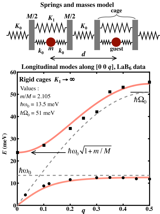
FIG. 2. Upper part, a classical chain of springs (stiffnesses k_0 , K_0 ) and masses ( m for the guest and M for the cage) for describing longitudinal modes in cage systems, including a cage stiffness K_1 . Lower part, the inelastic neutron scattering data for LaB 6 , from Ref. [29], confronted with computed dispersion curves (full lines) in the limit of perfectly rigid cages (see Appendix A). The dashed lines represent the underlying flat local mode of the guest, at frequency \omega_0 , and acoustic branch for empty cages with maximum frequency \Omega_0 .
