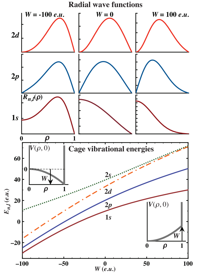
FIG. 6. Zero-temperature effect of the spherical well quadratic bottom, defined by the constant W . Lower part: energies of the four lowest oscillator levels 1s , 2p , 2d , and 2s , as functions of W with the insets representing, as functions of the reduced radius \rho , wells for positive and negative W . The CEF contribution results in a \beta shift of W toward negative values. Upper part: sketches of the radial wave functions for the 1s , 2p , and 2d states, for a flat bottom ( W = 0 ) and for opposite strong convexities ( W = 100 and -100 e.u. ).
