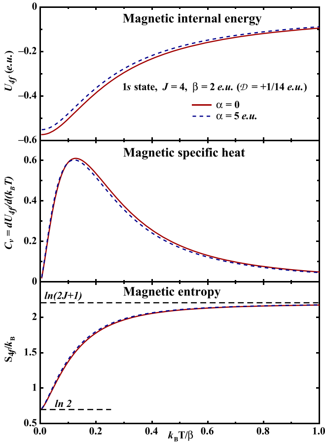
FIG. 4. Computed thermodynamic consequences, as function of the reduced temperature k_B T/\beta , for a cage split J = 4 multiplet in the spherical 1s vibrational ground state. The full line curves are obtained for a nonmagnetic potential with flat bottom ( \alpha = 0 ), whereas the dashed lines are for a quadratic bottom ( \alpha = 5 e.u.). \beta is the amplitude of the energy decrease for the lowest CEF level at the cage limit. The upper part gives the temperature variation of the 4f shell contribution to the internal energy. The middle and lower frames, respectively, show the associated specific heat and magnetic entropy.
