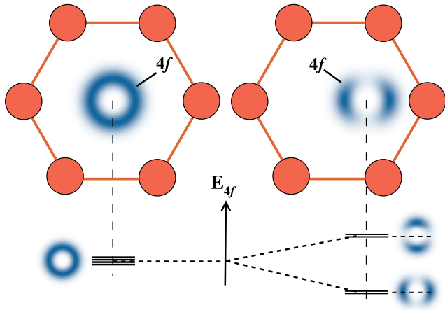
FIG. 1. Schematic illustrating the effect, inside a high-symmetry cage, of an off-center position for a rare-earth ion ( R^{3+} ) with a non-Kramers CEF ground level. Outside the cage center, the non-Kramers level is split (energy scale E_{4f} ). At low temperature, the off-center position and its altered 4f electrons distribution (schematized densities) are statistically favored.
