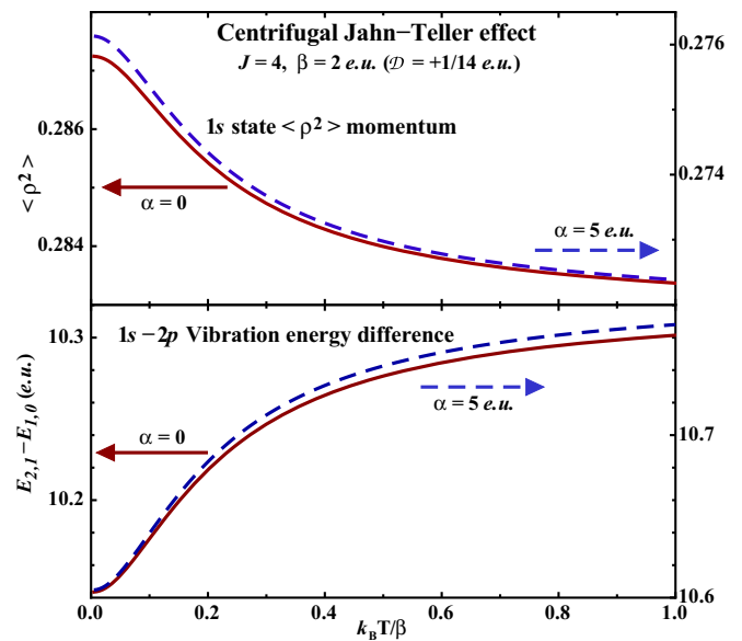
FIG. 7. Illustrations of the centrifugal Jahn-Teller effect in the spherical simplification within the 1s state, for J = 4 , \beta = 2 e.u. and two values, 0 (full lines) and 5 e.u. (dashed lines), of \alpha . The upper part materializes the centrifugal effect via the temperature dependence of the second-order radial moment \langle \rho^2 \rangle for the cage guest. The lower part shows the softening effect on the energy difference between the lowest vibration levels 1s and 2p . The left vertical scales are for the flat bottom case, \alpha = 0 , whereas the right ones are for \alpha = 5 e.u. . Left and right scales do not differ in amplitude, but are adapted by a shift.
