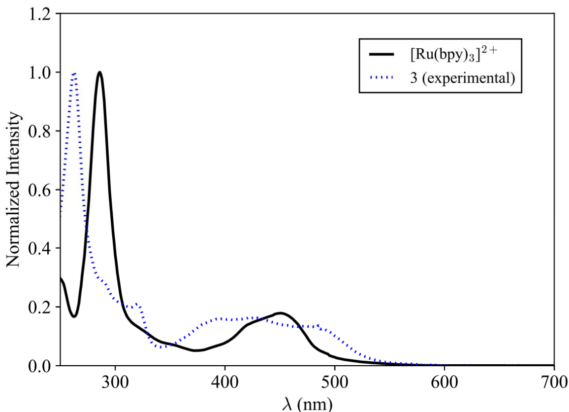
Figure 2. Normalised absorption spectrum of 3 and [\text{Ru}(\text{bipy})_3]^{2+} in \text{CH}_3\text{CN} .
