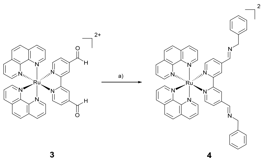
Scheme 2. Synthesis of conjugate 4 . a) benzylamine, EtOH, 50°C for 2 h under \text{N}_2 atmosphere, 54%.
