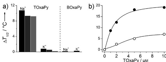
Figure 1. a) Left: Stabilization of F21T (0.2 \mu M ) by TOxapy (1 \mu M ) alone (black bar) and in presence of ds26 (3 and 10 \mu M , dark and light gray bars) in Na^+ - or K^+ -rich buffer. Right: stabilization of F21T by BOxapy (1 \mu M ) in the indicated cationic conditions. b) Stabilization of F21T as a function of TOxapy concentration in Na^+ ( \bullet ) and K^+ -rich ( \circ ) buffer (composition of the Na^+ - and K^+ -rich buffers is specified in the Supporting Information). The y axis label in (a) also corresponds to (b).
