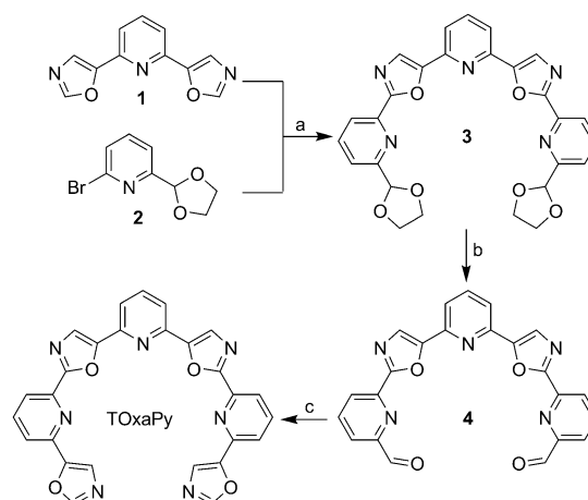
Scheme 3. Regiospecific synthesis of TOxapy a) CuI, Pd(OAc)_2 , Cs_2CO_3 , PCy_3 \cdot HBF_4 , dioxane, 130 °C, 24 h (45%); b) HCl (2 M), 110 °C, 2 h, (84%); c) TosMIC, K_2CO_3 , MeOH, 50 °C, 16 h (50%).
