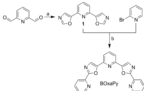
Scheme 2. First approach affording BOxapy and TOxapy as a mixture of isomers. a) TosMIC, K_2CO_3 , MeOH, 50 °C, 16 h (50%); b) CuI, Pd(OAc)_2 , Cs_2CO_3 , PCy_3 \cdot HBF_4 , dioxane, 130 °C, 24 h (45%); TosMIC = p -toluenesulfonylmethyl isocyanide; Cy = cyclohexyl.
