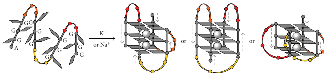
FIGURE 1: Schematic representation of the folding of an oligonucleotide that mimics the human telomeric sequence (d[AG 3 (T 2 AG 3 ) 3 ]). The polymorphism of the quadruplex is represented through the various possible structures, namely, the hybrid (left), antiparallel (centre), and parallel (right) forms; these structures differ by strand orientation (grey dashed arrows) and loop arrangement (represented in orange, yellow, and red).
