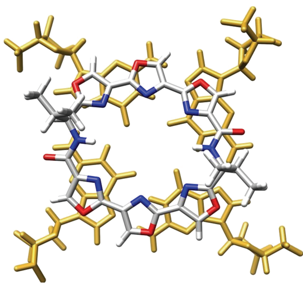
FIGURE 5: Qualitative in silico superposition of HXDV and a G-tetrad (extracted from PDB entry: 2A5R); guanine residues appear in gold, the carbon, nitrogen, oxygen, and hydrogen atoms of HXDV in grey, blue, red and white, respectively.
