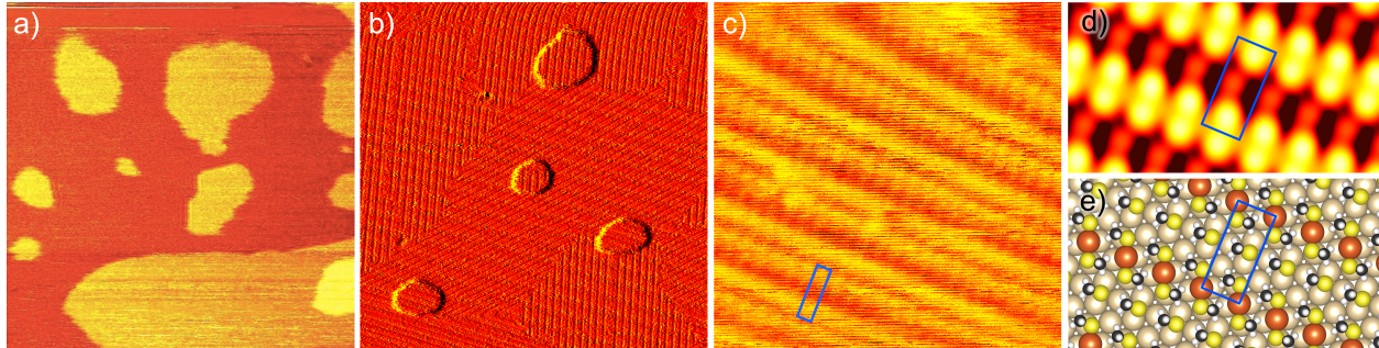
Figure 4: Structure of methanethiolate SAM at 1 bar ( P_{\text{CH}_3\text{SH}} = 1000 mbar, P_{\text{H}_2} = 0.35 mbar), 383 K. a) Au adatom islands shortly after transition to 1 bar ( 80 \times 80 nm 2 , U_s = -0.2 V, I_t = 120 pA). b) SAM structure on adatom islands. The STM image was differentiated to visualize the SAM structure on both the terrace and the adatom islands ( 80 \text{ nm} \times 80 \text{ nm} , U_s = -0.1 V, I_t = 800 pA). c) Details of SAM structure, 10 \times 10 nm 2 , U_s = -0.1 V, I_t = 800 pA. Corrugation in SAM structure: 0.02 nm. d) Simulated STM image (-1V, 500 pA, corrugation: 0.08 nm) for the structure in c), and e) The corresponding ball model.
