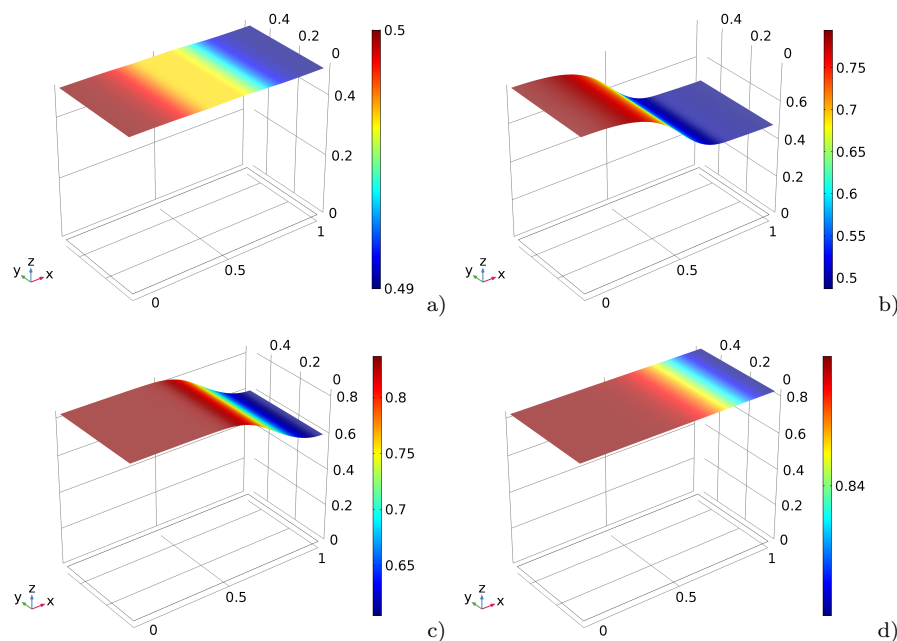
Fig. 17 Normalized mass density. a) initial stage; b) bone growth in the healthy zone; c) growth of new bone in the necrotic zone; d) final stage.
