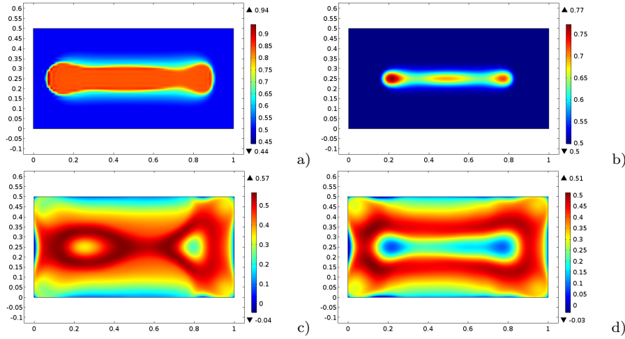
Fig. 7 Normalized mass density for the nonlocal instantaneous model of stimulus under uniform tension load at the end of simulation: a) 1.5F_H ; b) 1.3F_H ; c) 0.4F_H ; d) 0.3F_H .
