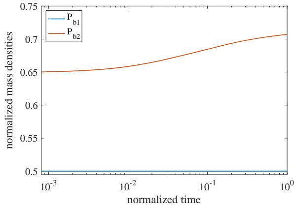
Fig. 14 Time history of the apparent bone mass density in two probe points located at the center P_{b1} and near a long side of the sample P_{b2} for the non-uniform tension test with the nonlocal instantaneous model of stimulus. The normalized time is represented in logarithmic scale.
