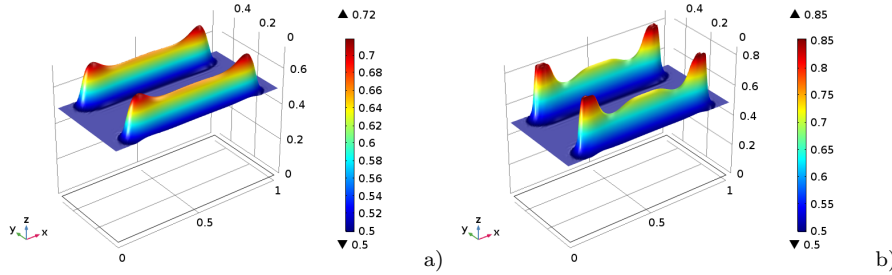
Fig. 15 Normalized mass density in non-uniform tension test with the nonlocal instantaneous model of stimulus. a) intermediate stage; b) final stage.
