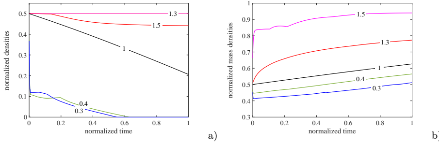
Fig. 8 Time history of the apparent bone mass density with the nonlocal instantaneous model of stimulus under uniform tension load: a) minimum value; b) maximum value.
