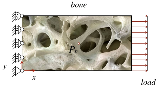
Fig. 4 Uniform extension test: a physiological case.
