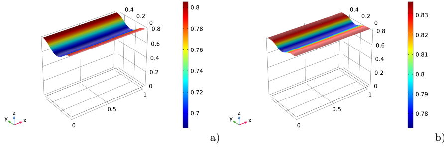
Fig. 12 Normalized mass density in non-uniform tension test with the diffusive model of the stimulus. a) intermediate stage; b) final stage.
