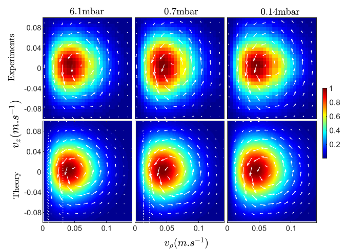
FIG. 1. Experimental and theoretical probability currents \bar{\mathbf{J}}_{\mathbf{v}} in velocity space for several pressures in the (radial v_{\rho} , axial v_z ) plane. The theory is described in the companion article [20]. The color bar displays the steady-state probability distribution P_s(\mathbf{v}) .
