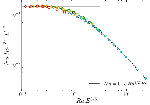
FIGURE 7. Nusselt number compensated by Ra^{3/2}E^{-2} as a function of RaE^{8/5} . Only the cases with E \leq 3 \times 10^{-4} and Nu \geq 2 are displayed in this figure. The solid black line corresponds to the diffusivity-free scaling Nu = 0.15 Ra^{3/2}E^2 (Equation 3.8) already displayed in figure (5), while the vertical line corresponds to the dynamical boundary scaling RaE^{8/5} = 0.4 . The symbols have the same meaning as in figure 1.
