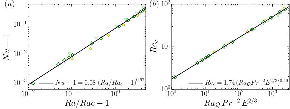
FIGURE 3. (a) Nusselt number Nu - 1 as a function of Ra/Ra_c - 1 . (b) Reynolds number Re_c as a function of Ra_Q Pr^{-2} E^{2/3} . Only the cases with E \leq 3 \times 10^{-5} and Ra \leq 6 Ra_c are displayed in this figure. In both panels, the solid black lines correspond to the least-square fits to the data. The symbols have the same meaning as in figure 1.
