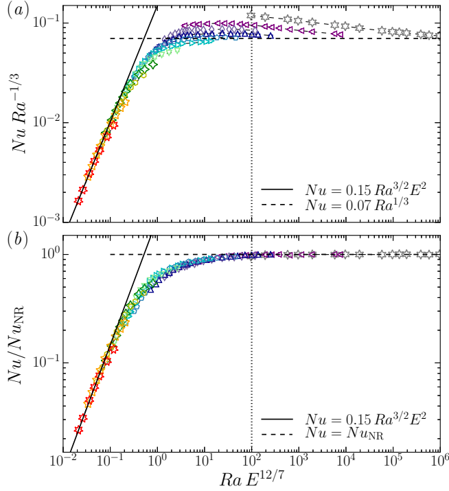
FIGURE 16. (a) Nusselt number Nu renormalised by Ra^{1/3} as a function of RaE^{12/7} (Equation 3.26). The solid black line corresponds to the asymptotic scaling for rotating convection (3.8), while the dashed line corresponds to the tentative asymptotic scaling for non-rotating convection. (b) Nusselt number Nu renormalised by Nu_{NR} as a function of RaE^{12/7} . Nu_{NR} corresponds to the Nusselt number of the non-rotating cases at the same Rayleigh number. On both panels, the weakly non-linear cases with Nu < 2 have been excluded. The dotted vertical lines correspond to the Rayleigh number Ra = 100 E^{-12/7} beyond which Nu adopts a scaling behaviour close to the non-rotating RBC. The symbols have the same meaning as in figure 1.
